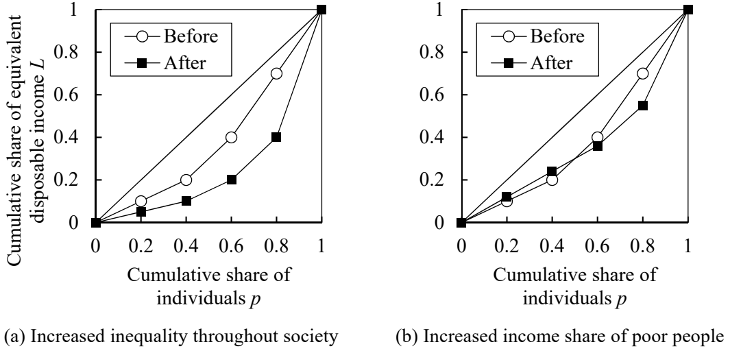
Figure 2.1 Examples of changes in Lorenz curves
