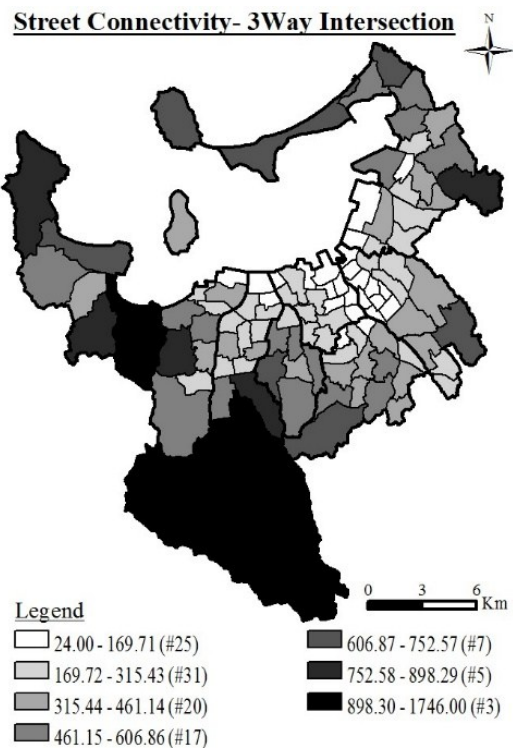
Figure 2.8 D3- 3way road intersection
