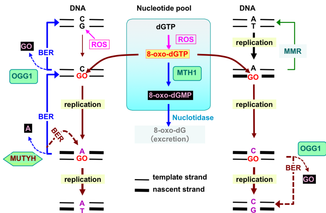
Fig. 1. Oxidation of guanine and defense mechanisms to minimize its accumulation in DNA.
