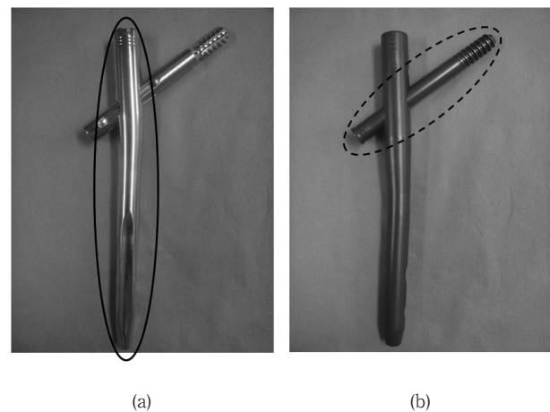
Fig. 1 Photographs of the angled cephalomedullary device of the proximal femur. (a) The device made of stainless steel. (b) The device made of titanium alloy. The solid circle is the rod, and the dotted circle is the lag screw. The angle between the rod and the lag screw was 130°.
