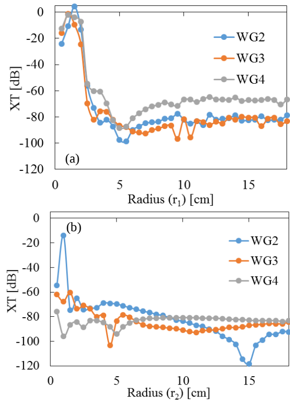
Fig. 3. Relation between crosstalk and (a) radius r_1 , (b) radius r_2 with light input to WG1
