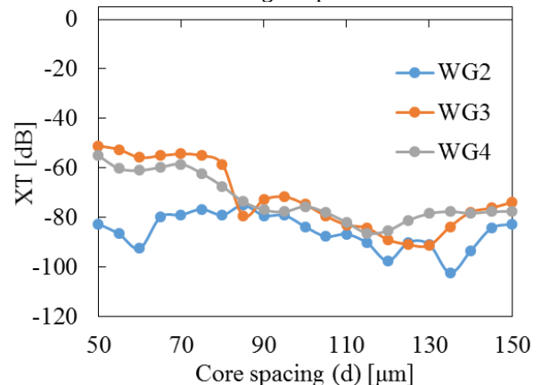
Fig. 4. Crosstalk and core spacing ( d ) relation
