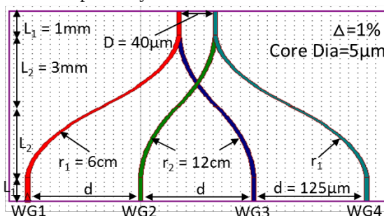
Fig. 2. Two dimensional view of 3D waveguide structure with all dimensions
