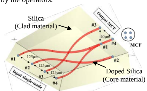
Fig. 1. Structure of the proposed device
