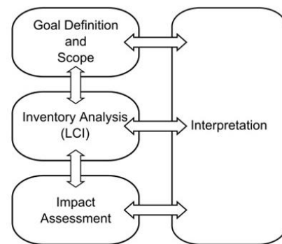
Fig. 5. LCA framework [8]
