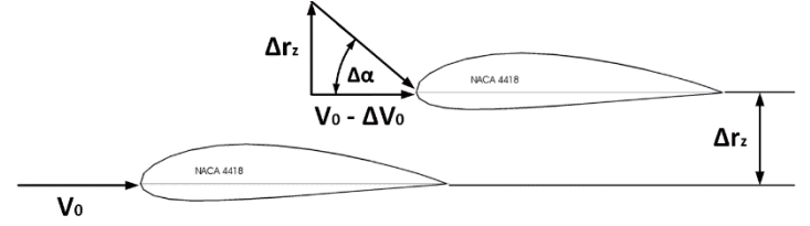
Figure 15. Illustration of AOA variation.
