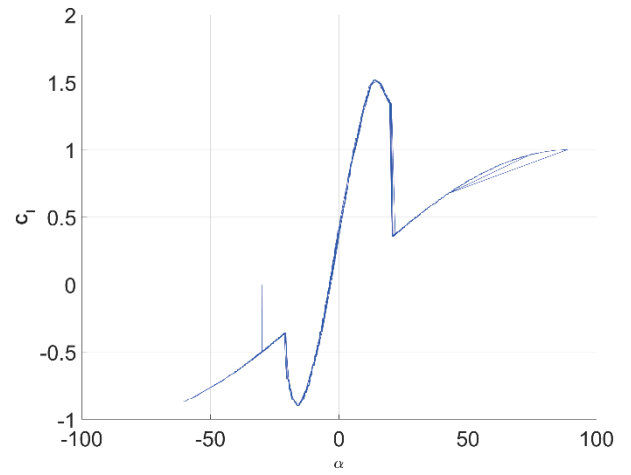
Figure 16. C_l - \alpha curve generated from code for validation
