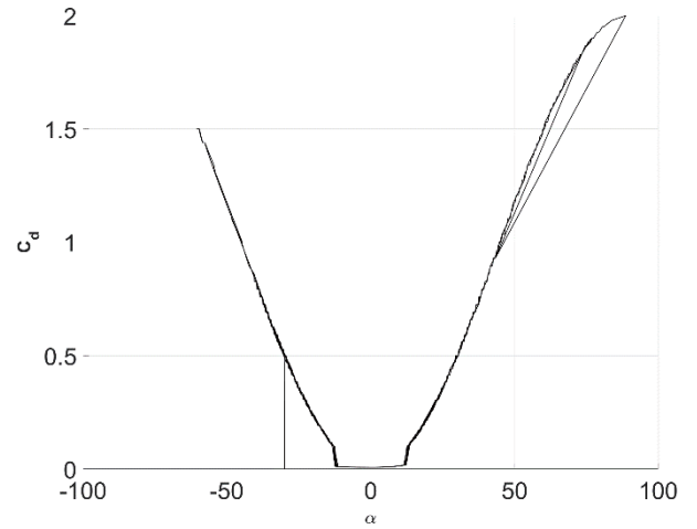
Figure 17. C_D - \alpha curve generated from code for validation.
