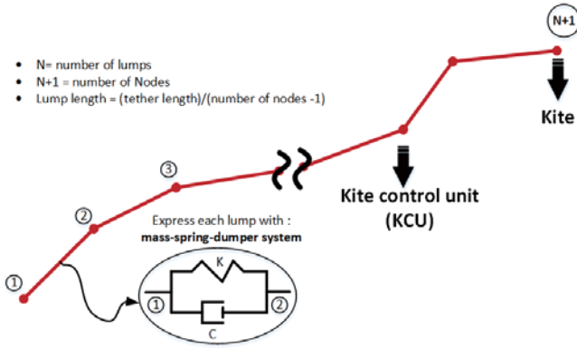
Figure 3. Overview of the simulation procedure.
