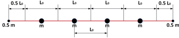
Figure 1. Illustration of mass distribution for LLM of 5 lumps.
