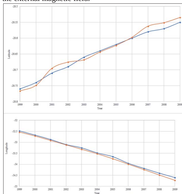
Figure 6: Secular variation of the latitudinal (top) and longitudinal (bottom) B_{\min} position of the SAA using IGRF model
