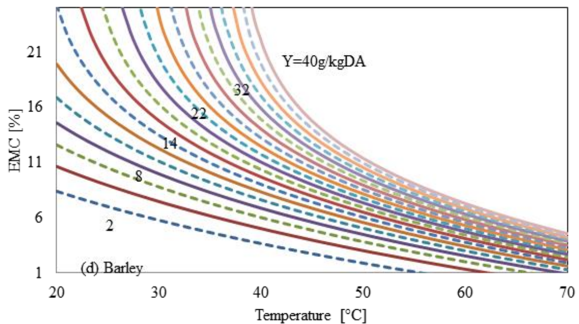
Figure 3.1 (b) Effect of temperature and humidity ratios on EMC for barley and corn.
