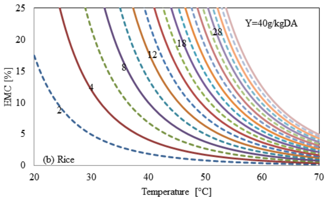
Figure 3.1 (a) Effect of temperature and humidity ratio on EMC for wheat and rice.
