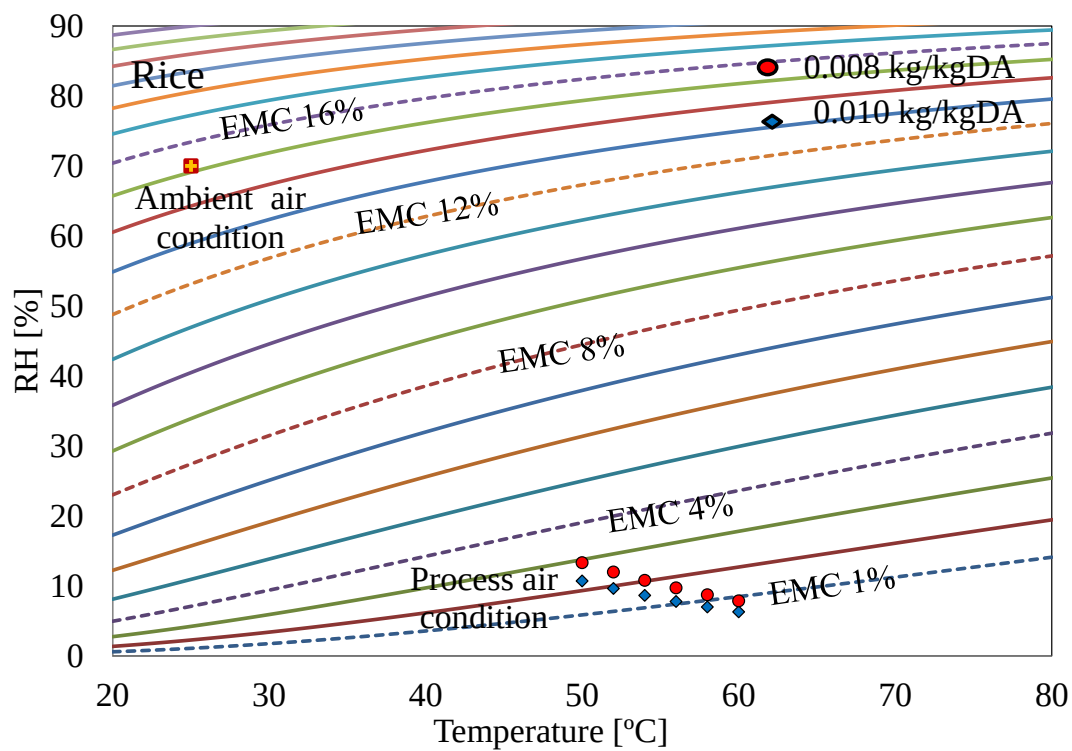
Figure 3.8 (a) Pictorial representation of process air conditions at different levels of air heating on EMC chart for Case-II for wheat and rice.
