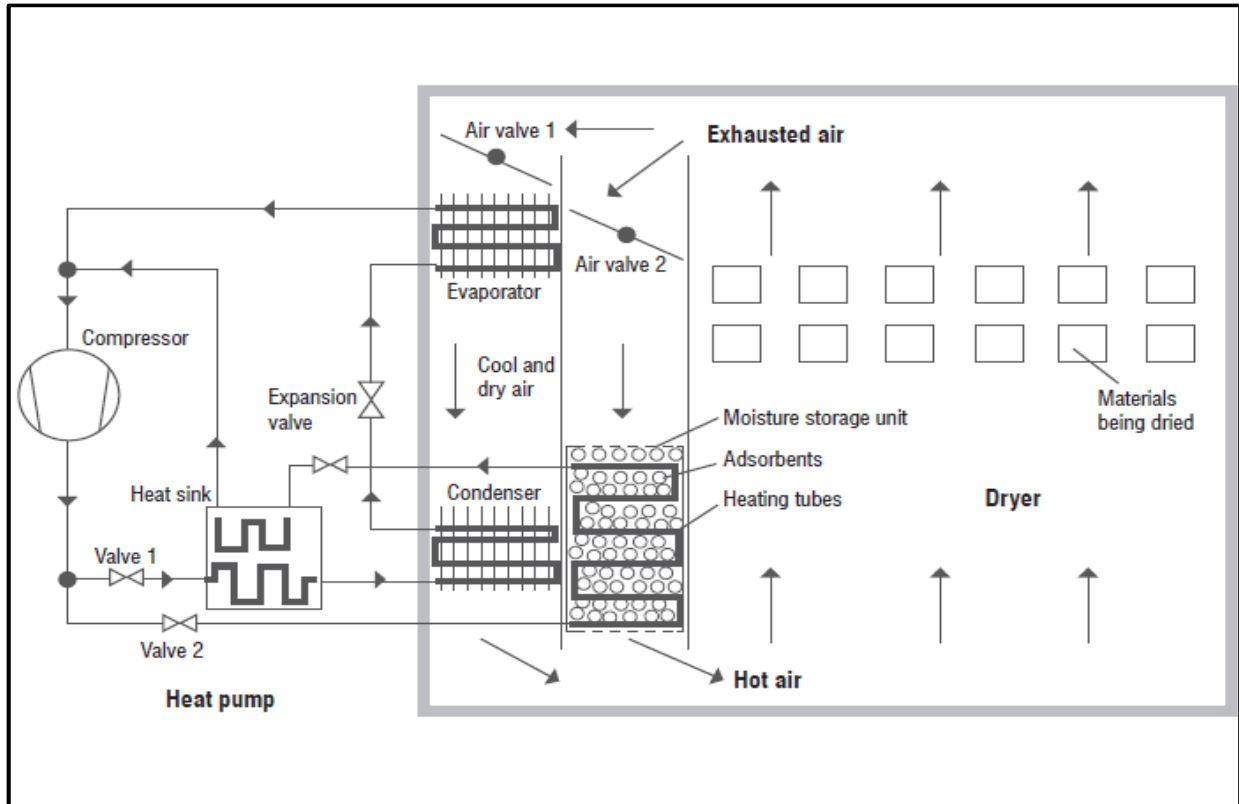
Figure 2.8 Desiccant assisted heat pump dryer (Kivevele and Huan 2014).
