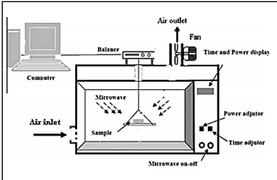
Figure 2.3 Schematic diagram of microwave-convective oven dryer (Zarein et al., 2015).
