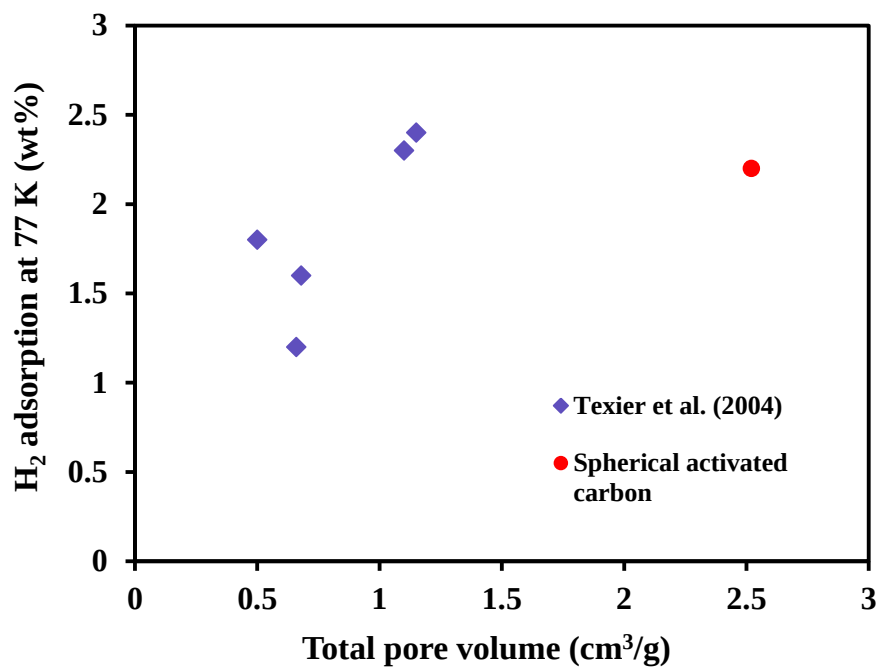
Figure B.3 H_2 adsorption at 1 bar and 77 K with total pore volume.
