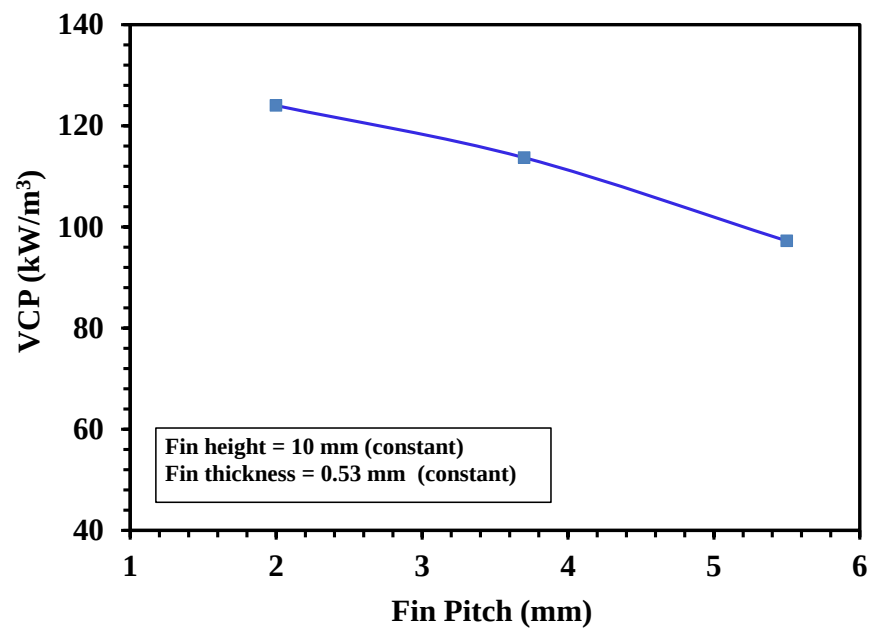
Figure 5.11 Effect of fin pitch variation on volumetric cooling power (VCP).
