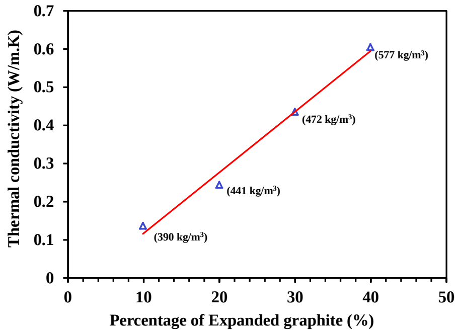
Figure 3.4 Thermal conductivity improvement with the percentage increase of expanded graphite (El-Sharkawy et al., 2016).
