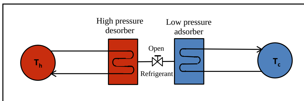
Figure 1.6 Conceptual diagram of mass recovery cycle.
