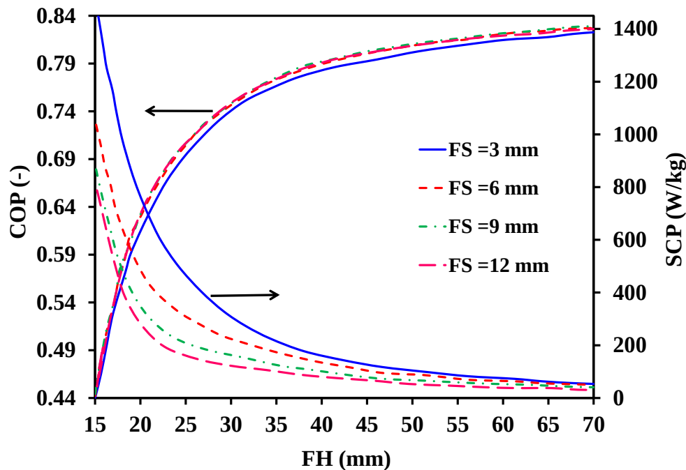
Figure 3.5 Effects of heat exchanger parameters on COP and SCP (Mahdaviikhah & Niazmand, 2013).
