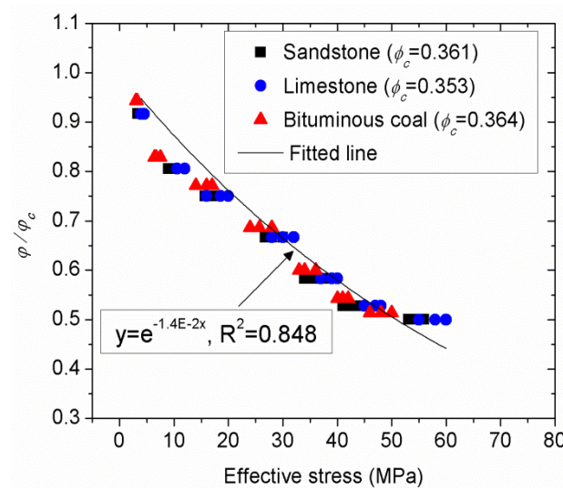
Figure 2-10. Effective stress versus porosity.
