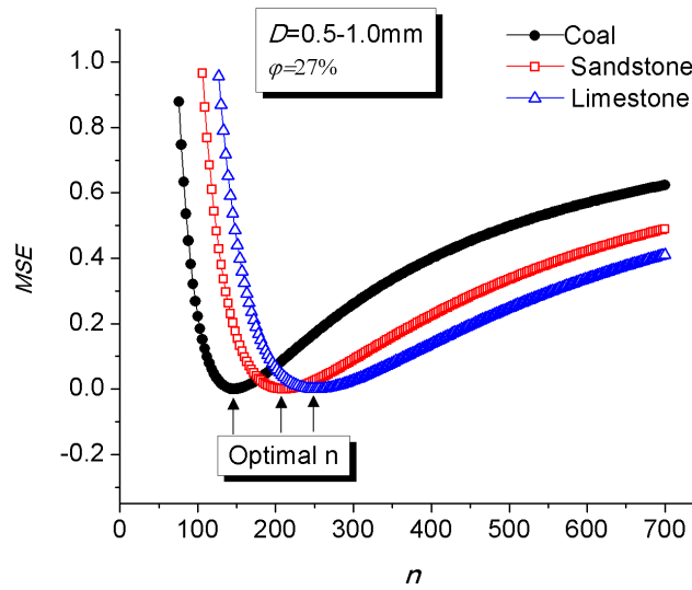
Figure 3-5. Mean squared error between the B-R model and measurement results vs. duplication factor, n , for compressed porous samples ( \phi = 0.27 ; D = 0.5\text{--}1.0 mm).
