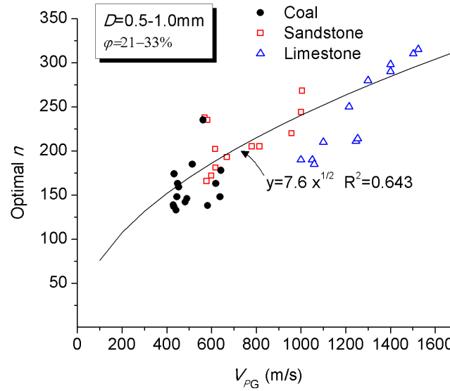
Figure 3-6. Correlation between optimal n and V_{PG} ( \varphi = 0.27-0.33 ; D = 0.5-1.0 mm).
