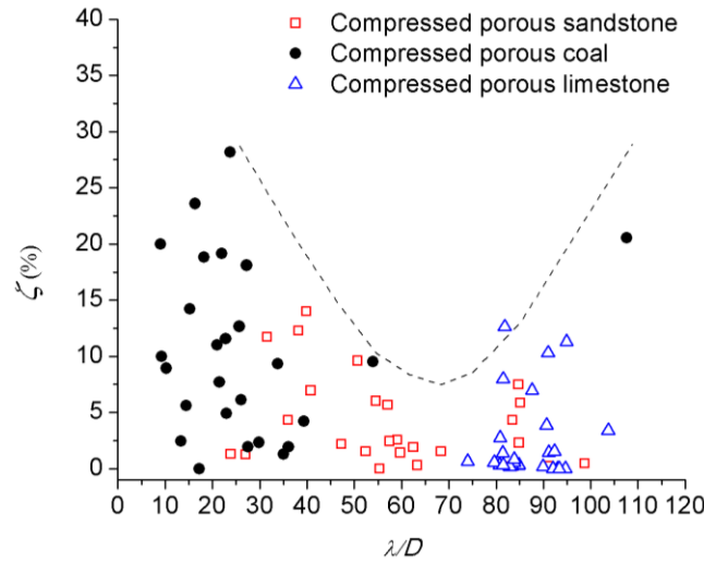
Figure 3-8. Difference error \zeta (%) between the measured data and the B-R model prediction vs. \lambda/D .
