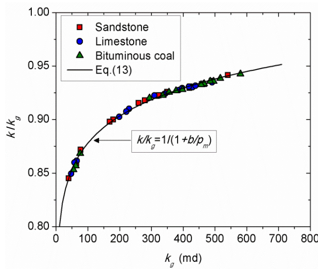
Figure 2-19. Correction of gas permeability.
