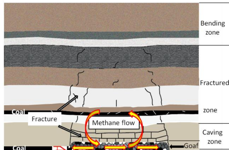
Figure 1-7. Methane flow in the goaf and the interaction with adjacent areas.
