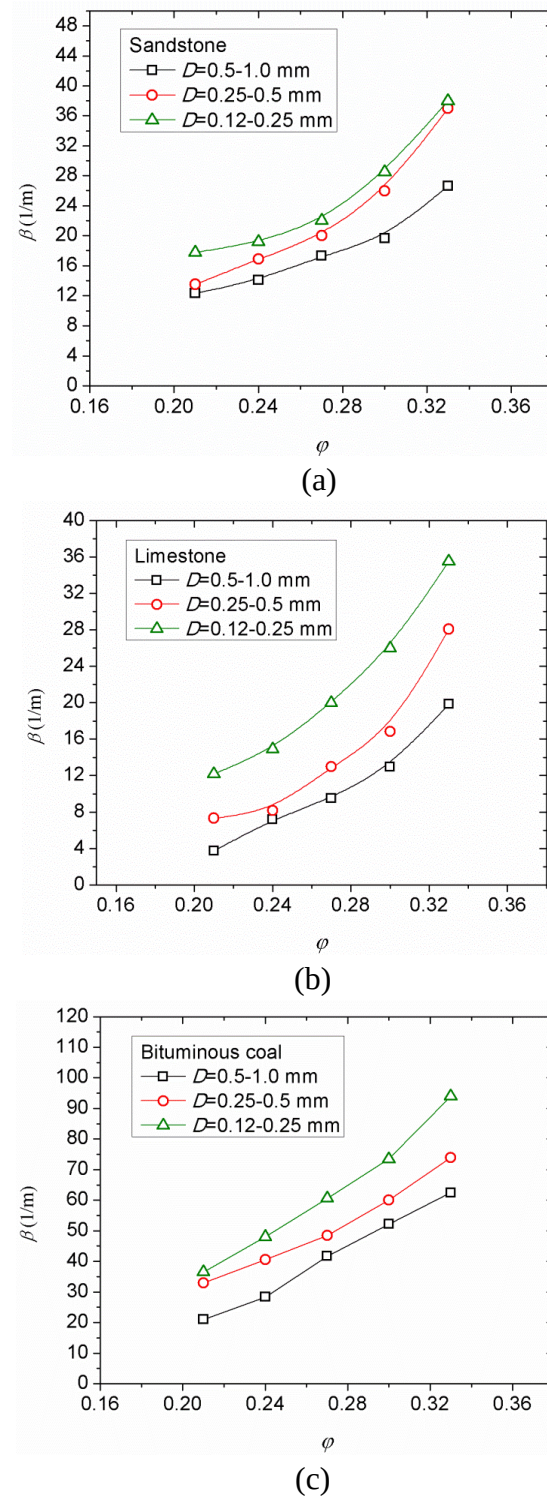
Figure 2-16. Seismic attenuation against porosity for different particle size. (a) sandstone, (b) limestone and (c) bituminous coal
