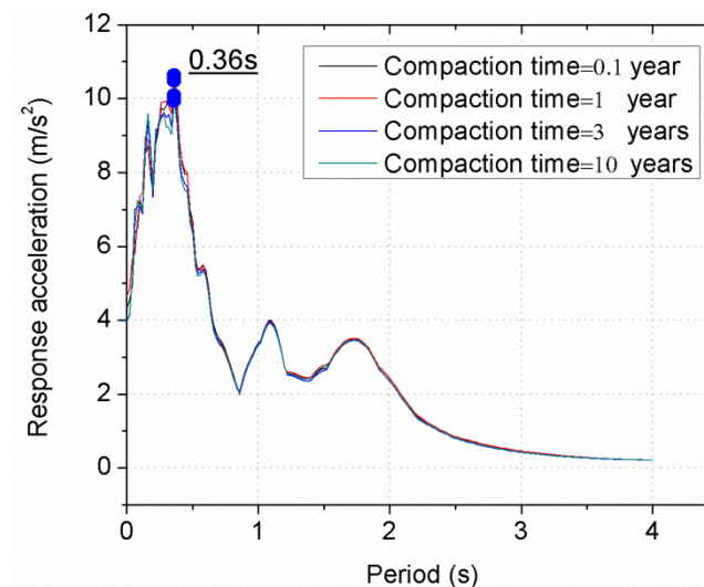
Figure 5-20. Response acceleration spectrum of point #1 above a 100m-depth-goaf for the cases of different compaction time.
