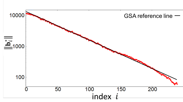
FIGURE 3.3: Semi-log graph of \|\mathbf{b}_i^*\| of a 240-dimensional highly reduced basis
