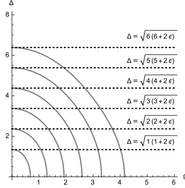
Figure 3.1: Curve P_6^{(6,\varepsilon)}((2g)^2, \Delta^2) = 0 with \varepsilon = 0.4 (for g, \Delta > 0 )
