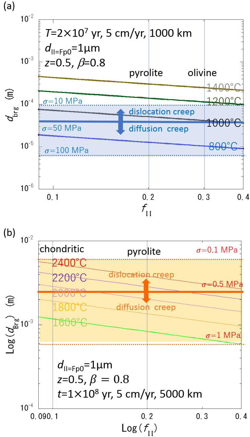
Fig. 2.17 Effects of the volume fraction of the secondary phase (ferropericlas) on the grain-size evolution of bridgmanite under the lower-mantle slab (a) and the lower mantle (b) conditions.
