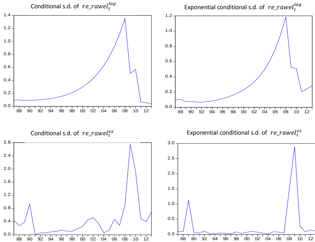
Figure 2.5 Conditional Standard Deviation
