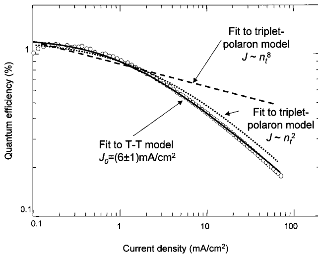
FIG. 13. The external quantum efficiency of the \text{Eu}(\text{TTA})_3\text{phen}:\text{CBP} device. It exhibits a roll-off characteristic of T - T annihilation with an onset current density of J_0 = 6 \pm 1 \text{ mA cm}^{-2} . The expected behavior of polaron-triplet quenching for bulk-limited transport ( J \propto [n_t]^8 ) does not fit the data. However, good agreement is obtained for polaron-triplet quenching models where J \propto [n_t]^2 .
