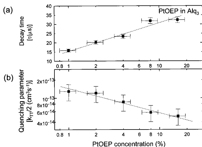
FIG. 8. The lifetime ( \tau ) and biexcitonic quenching rate ( k_{TT} ) as a function of the concentration of PtOEP in \text{Alq}_3 . The data are from an electroluminescent device with a high initial triplet concentration of [M^*(0)] \sim 1 \times 10^{18} \text{ cm}^{-3} to minimize errors in the fit due to intensity-independent curvature in the transient decays. Note that contrary to expectations of concentration quenching, the lifetime of PtOEP increases with concentration. This is another example of the importance of PtOEP- \text{Alq}_3 interactions in this material system.
