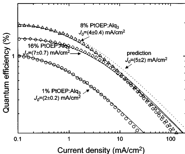
FIG. 9. External quantum efficiency of PtOEP: \text{Alq}_3 devices. The solid curves are fits to the data using Eq. (8) and demonstrate good agreement with behavior expected for biexcitonic quenching. The only deviation occurs at high current densities ( \sim 100 \text{ mA/cm}^2 ) where saturation of PtOEP is first apparent. Transient parameters plotted in Fig. 7 are used to predict a threshold current for the 8% PtOEP:CBP device of J_0 = 5 \text{ mA/cm}^2 . The best fit to the data (dashed curve) yields J_0 = 4 \text{ mA/cm}^2 .
