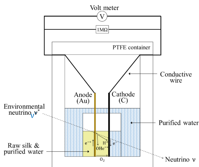
Fig. 1. Illustration of the low-energy environmental neutrino detector. Raw silk around an anode generates assisting field. When \nu^* enters into this region, it is supposed to dissociate water molecule into \text{OH}^- + \text{H}^+ .
