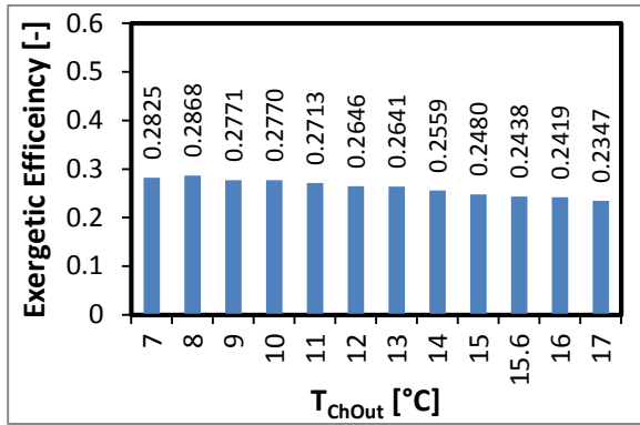
Fig. 4 Exergetic efficiency vs. T_{ChOut} at 32°C T_{CondIn}
