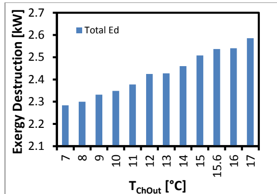
Fig. 7 Total Exergy Destruction vs. T_{ChOut} at 32°C T_{CondIn}
