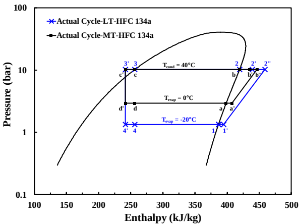
Fig. 1: P-h diagram of refrigeration cycles with suction gas superheating and liquid subcooling for HFC 134a for LT and MT; 4'-1 or d'-a: evaporation; 1'-1' or a-a': suction superheating; and 1'-2' or a'-b': compression; 2'-3 or b'-c: condensation; 3-3' or c-c': liquid subcooling; 3'-4' or c'-d': expansion
