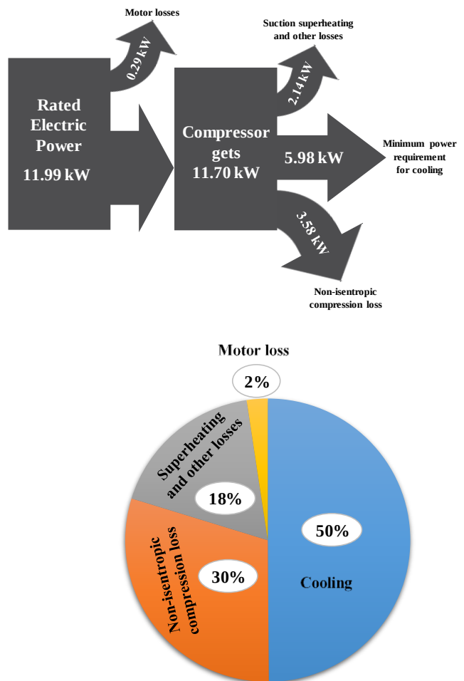
Fig. 4: Power distribution of a 27.7 kW (LT) compressor with HFC 134a refrigerant.
