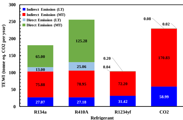
Fig. 2: TEWI for various refrigerants
