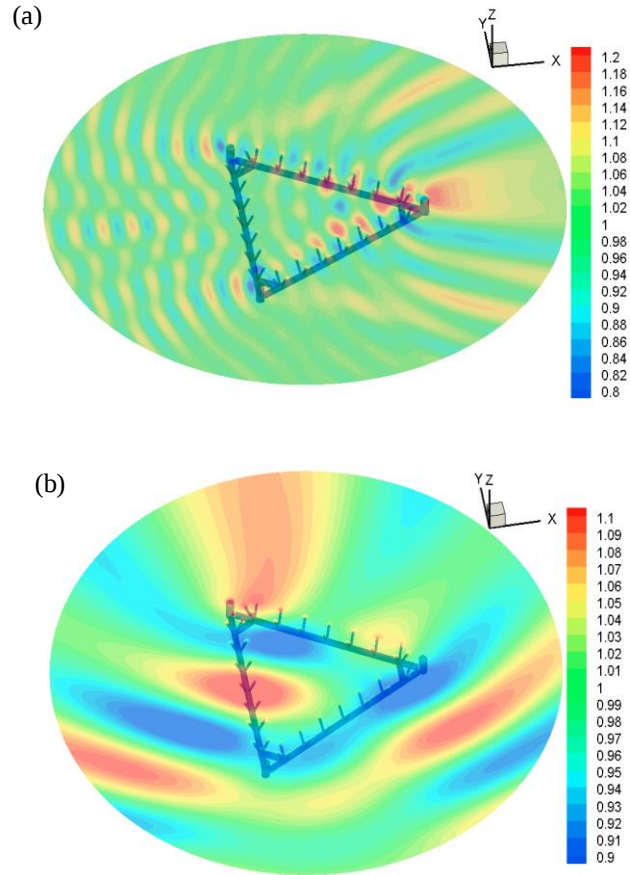
Fig. 5 Contour plot of free surface elevation (normalized by the incident wave amplitude) in the following conditions: (a) \alpha=0^\circ , kL=20.78 ; (b) \alpha=90^\circ , kL=5.16 . The upper column shows the free-surface elevation for a high frequency incident wave, while the bottom column shows the free-surface elevation for a low frequency incident wave.
