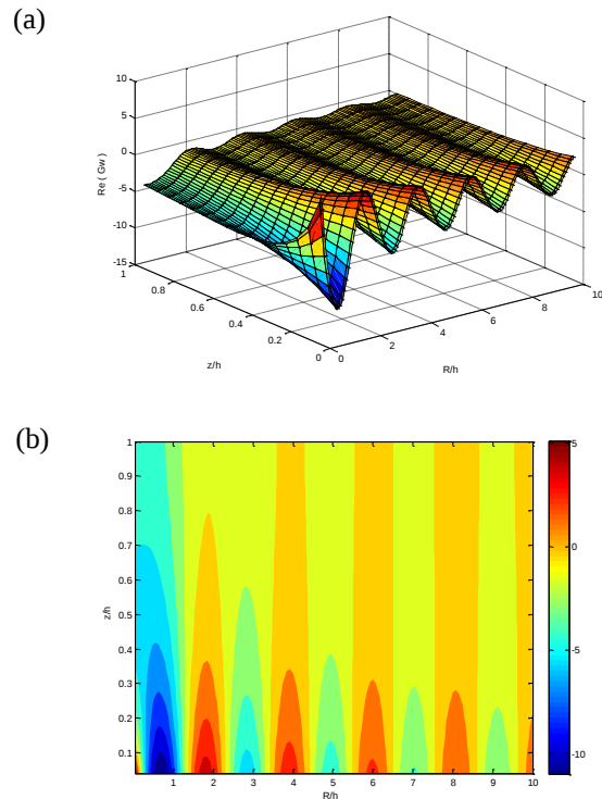
Fig. 3. Real part of the complex harmonic wave term Gw in free-surface Green's function, when a point source locates at the free surface with a pulsating frequency of f=8.6327 \times 10^{-1}\text{s}^{-1} : (a) oblique view, and (b) contour plot.
