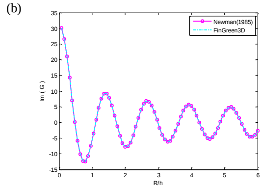
Fig. 2. Values of free-surface Green's function G , as a function of R/h , when the point source and the field point locate at the free surface with a pulsating frequency of f=1.1145\text{s}^{-1} : (a) real part of G ; (b) imaginary part of G .
