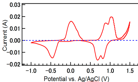
Fig. 4 Cyclic voltammogram of \text{LiMn}_2\text{O}_4 in 2 \text{ mol/dm}^3 \text{ Li}_2\text{SO}_4 aqueous solution with a scanning rate of 0.5 \text{ mV/s} .
