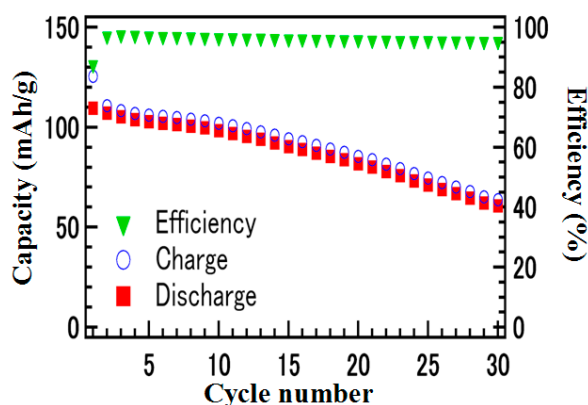
Fig. 8 Cyclability of symmetric cell with \text{LiMn}_2\text{O}_4 with 2 mol/dm 3 \text{Li}_2\text{SO}_4 aqueous solution at 50mA/cm 2 .
