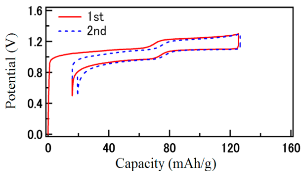
Fig. 6 Charge and discharge profile of \text{Li}_{1-x}\text{Mn}_2\text{O}_4//\text{Li}_{1+x}\text{Mn}_2\text{O}_4 with 2 mol/dm 3 \text{Li}_2\text{SO}_4 aqueous solution.
