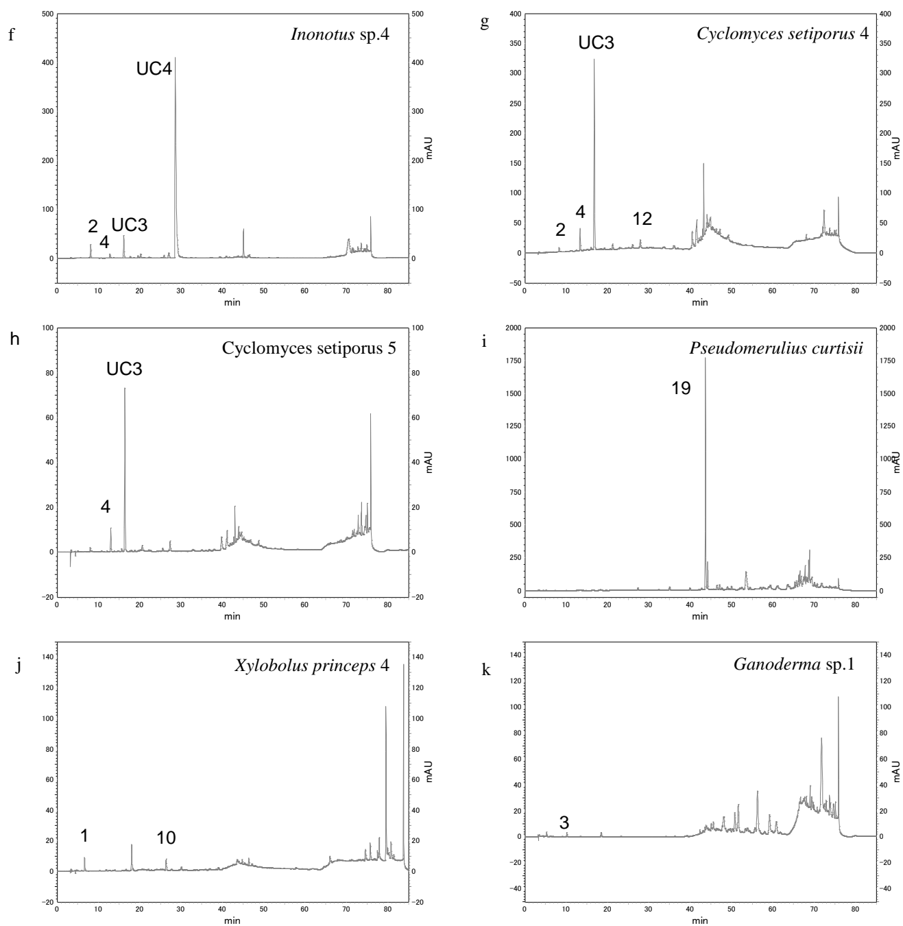
Figure A3.1. HPLC chromatograms at 280 nm of the standard compounds (a) and ethanol extracts of the top ten samples with the highest TPC (b to k). The peaks were identified as 1. 5-sulfosalicylic acid, 2. gallic acid, 3. pyrogallol, 4. 3,4-dihydroxybenzoic acid, 5. chlorogenic acid, 6. (+)-catechin, 7. p -hydroxybenzoic acid, 8. vanillic acid, 9. caffeic acid, 10. vanillin, 11. rutin, 12. p -coumaric acid, 13. ferulic acid 14. veratric acid, 15. naringin, 16. benzoic acid, 17. abscisic acid, 18. quercetin, 19. trans -cinnamic acid, 20. naringenin, 21. kaempferol
