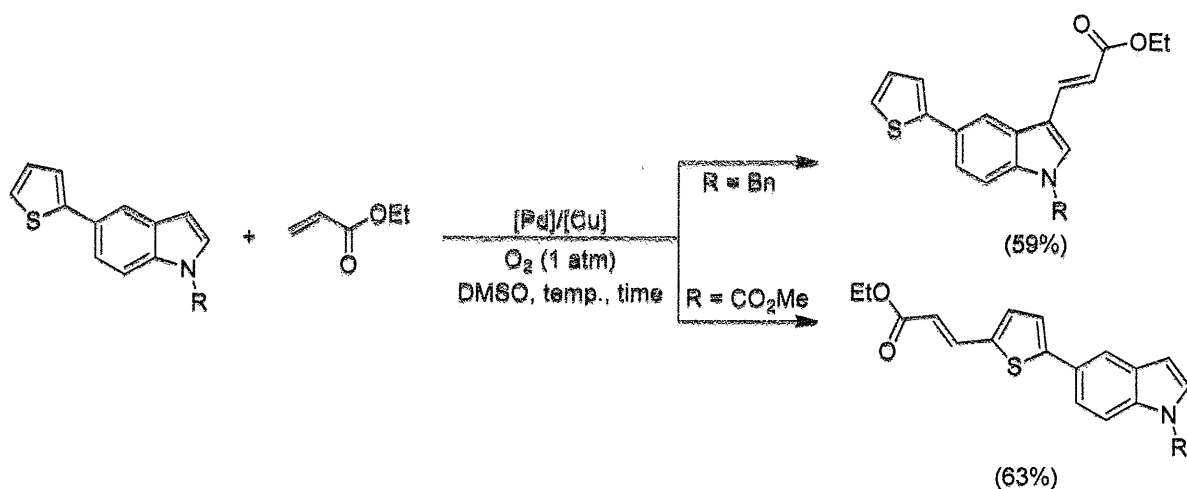
Scheme 1. Tuning Reactivity between Thiophene and Indole in a Single Molecule
