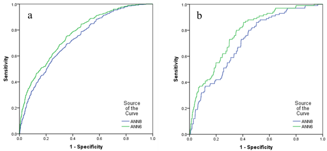
Figure 4.7 Receiver operating curves 6 factors and 8 factors artificial neural network methods. Figure 7a indicates success rate curves and Figure 7b indicates the prediction rate curve.
