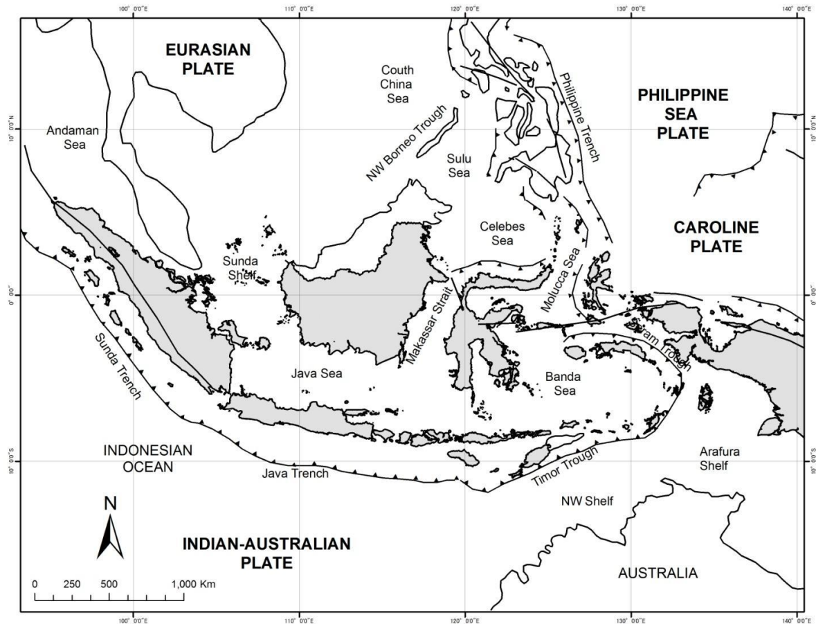
Figure 1.1 Indonesia regional tectonic setting
