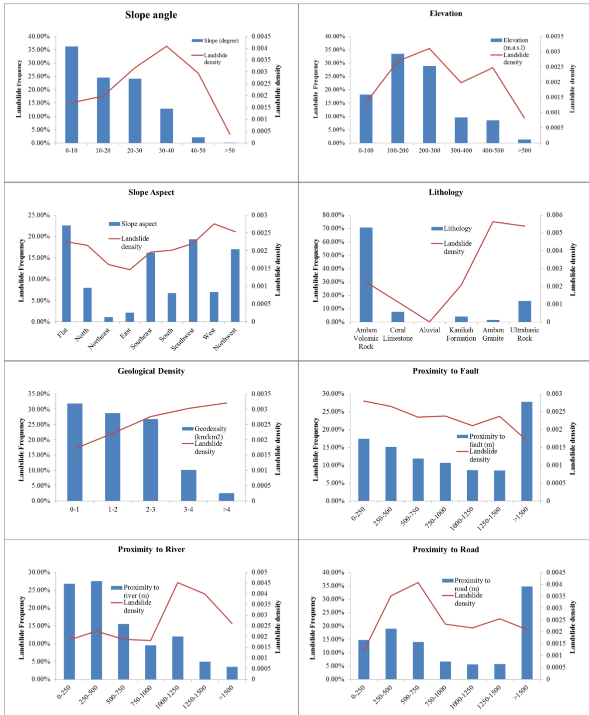
Figure 4.8 The eight causative factors relationship with landslide frequency and landslide density.
