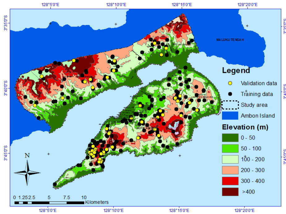
Figure 4.2 Landslide training and validation data in the study area.
