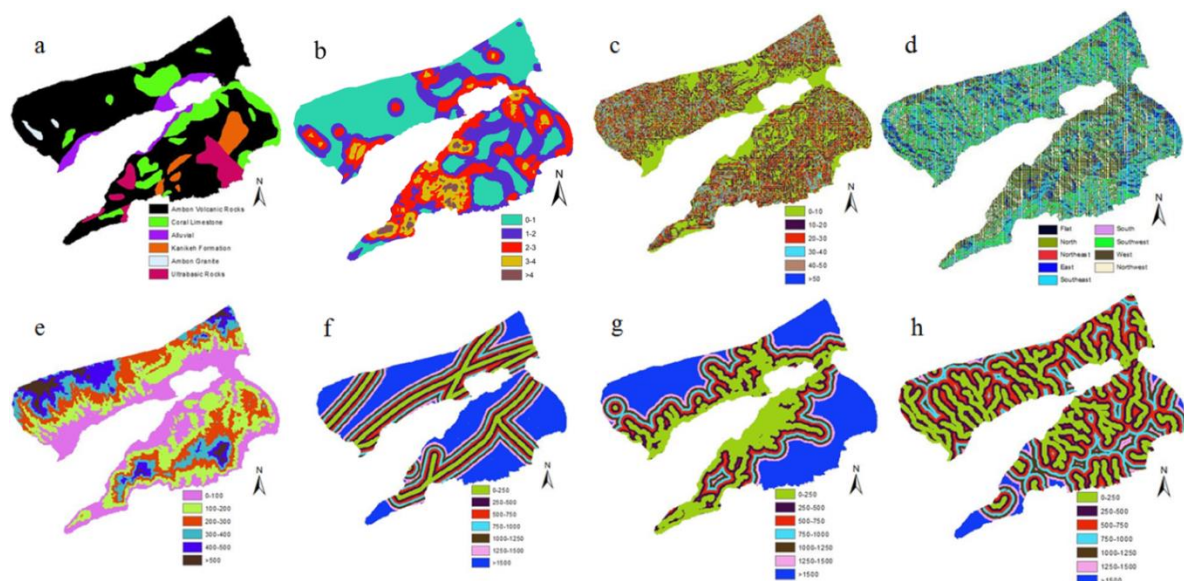
Figure 3.3 Distribution of the eight causative factors used as independent variables in this study. a) lithology; b) density of geological boundaries; c) slope; d) slope aspect; e) elevation; f) proximity to faults; g) proximity to road networks; h) proximity to river
