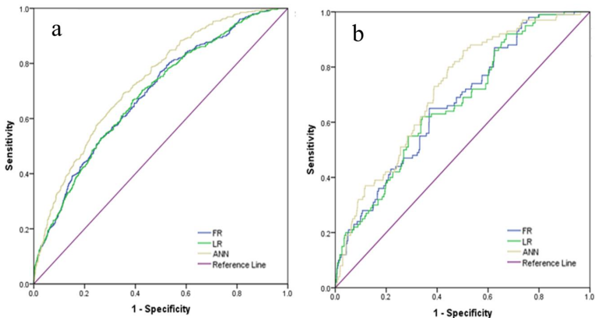
Figure 3.6 Receiver operating curves (ROC) for frequency ratio (FR), logistic regression (LR), and artificial neural network methods. Figure 3.6a indicates success rate curves and Figure 3.6b indicates prediction rate curves.
