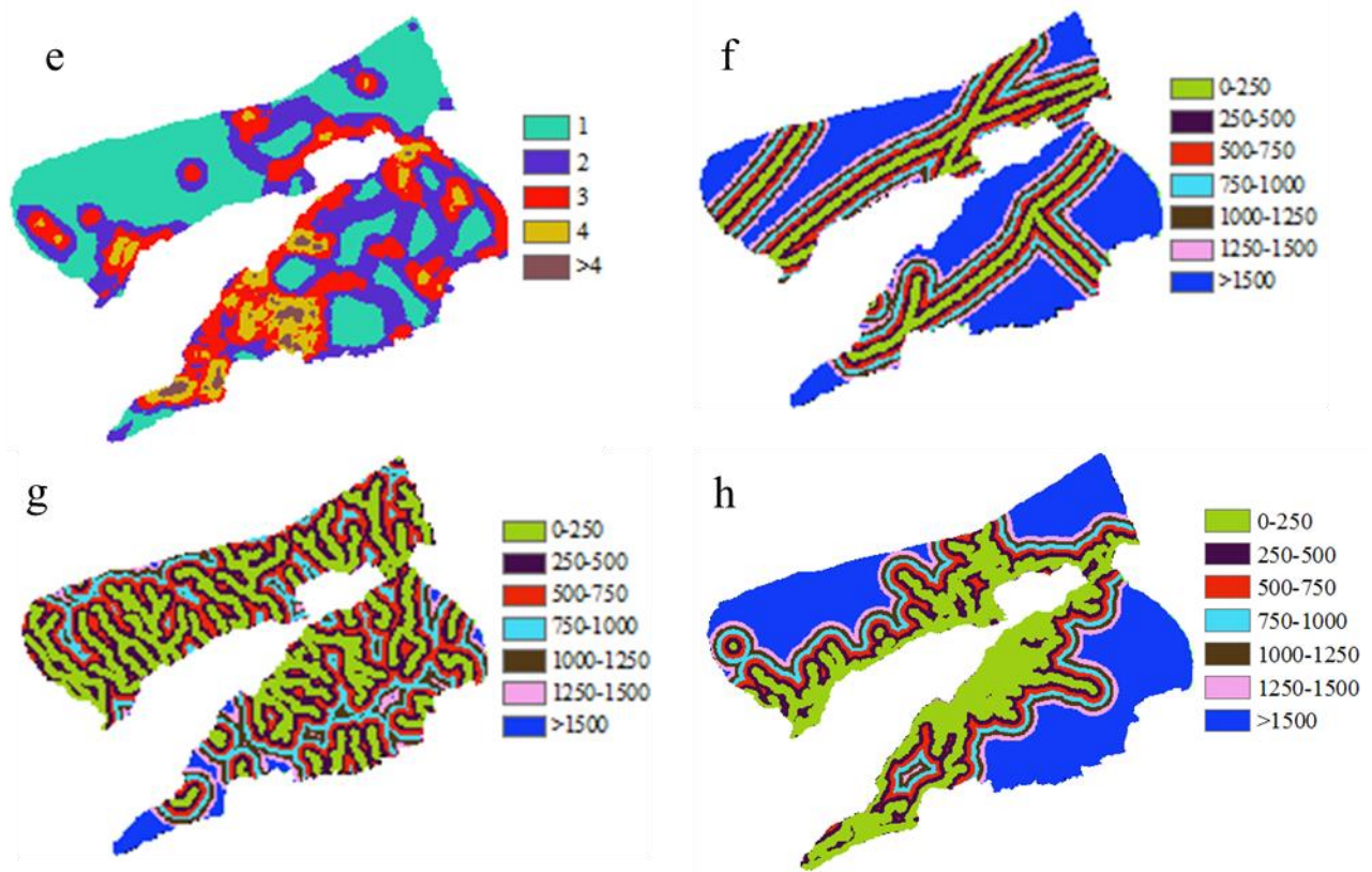
Figure 4.3 Distribution of the eight causative factors used as independent variables in this study. a) elevation; b) slope; c) slope aspect; d) lithology; e) geological density; f) proximity to faults; g) proximity to river; h) proximity to road networks.
