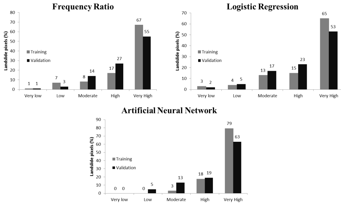
Figure 3.5 The ratio (%) of landslide pixels for each susceptibility class to the total landslide pixels for landslide sustainability maps based on training and validation data. Figure 3.5a, 3.5b, 3.5c were derived using frequency ratio, logistic regression, artificial neural network
