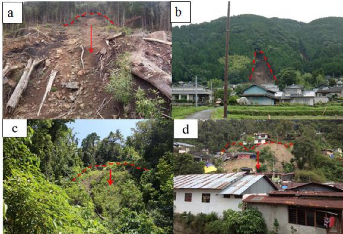
Figure 5.1 Pictures of landslide location in (a) Aso Teno; (b) Aso Nakasakanashi; (c) Ambon Eerie; (d) Ambon Seilale.
