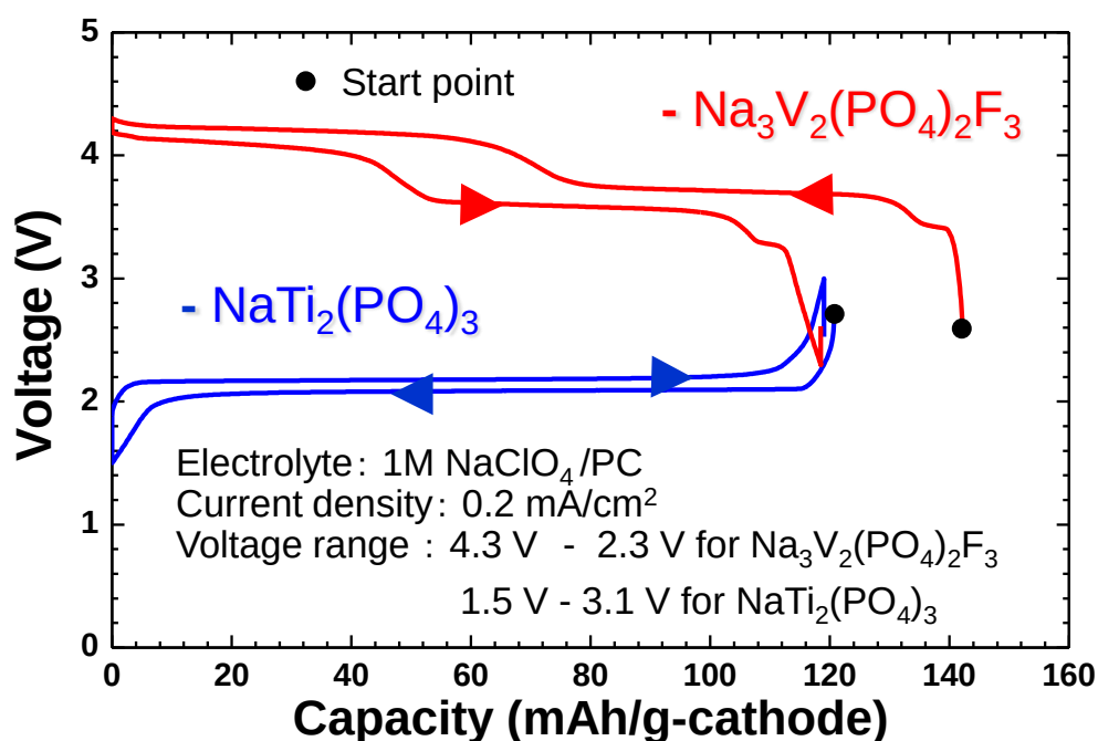
Figure 13 Charge and discharge profiles of \text{Na}_{3-x}\text{V}_2(\text{PO}_4)_3 and \text{Na}_{1+x}\text{Ti}_2(\text{PO}_4)_3 in Na cells.
