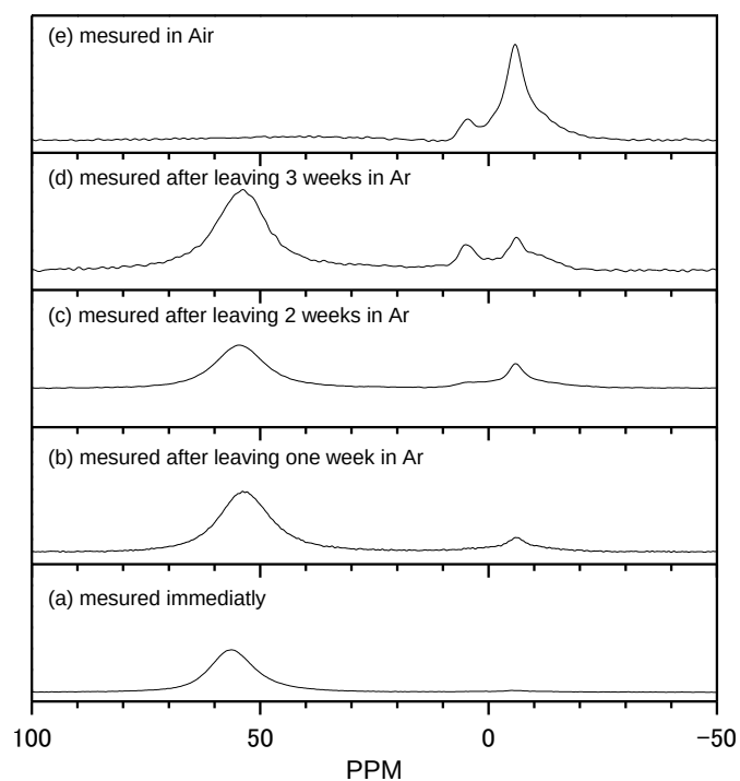
Figure 42. ^{23}\text{Na} NMR spectrum of discharged \text{Na}_2\text{C}_6\text{O}_6 sample for 1.25 V. The sample was (a) measured immediately after disassembling a cell, and left for (b) 1, (c) 2 and (d) 3 week in Ar glove box and measured in Ar condition, and (e) exposed in the air and measured in Air condition.
