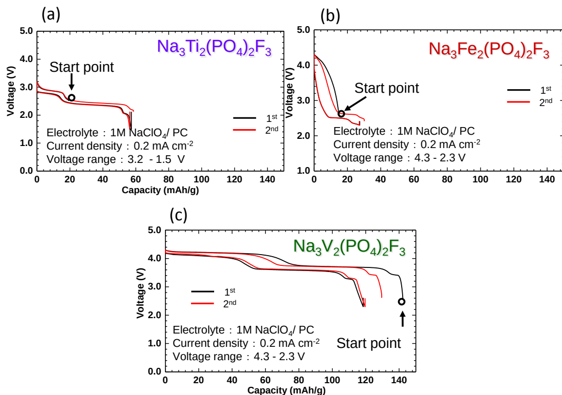
Figure 9. Charge and discharge profiles of \text{Na}_3\text{M}_2(\text{PO}_4)_2\text{F}_3 [ \text{M} = (a) Ti, (b) Fe, and (c) V] in Na cells.
