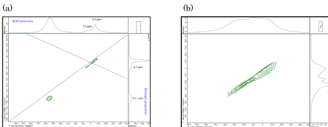
Figure 41. ^{23}\text{Na} MQMAS NMR spectrum for the \text{Na}_2\text{C}_6\text{O}_6 samples after being discharged for (a) 1.25 V and down to (b) 1.5 V.
