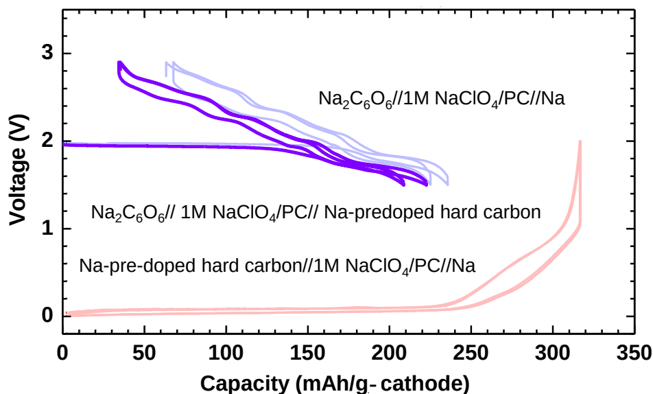
Figure 30. Charge and discharge profiles of \text{Na}_2\text{C}_6\text{O}_6//1\text{M NaClO}_4/\text{PC}//\text{Na} -predoped hard carbon. Voltage range and current density were set to 1.5 V – 3.0 V and C/20 based on 180 \text{mAh g}^{-1} . The charge and discharge profiles of \text{Na}_2\text{C}_6\text{O}_6 and Na-predoped hard carbon in Na cells are also presented as reference.
