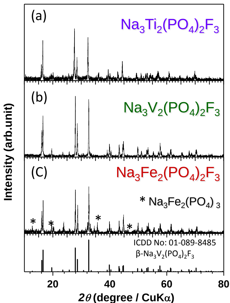
Figure 8. XRD patterns of (a) \text{Na}_3\text{Ti}_2(\text{PO}_4)_2\text{F}_3 , (b) \text{Na}_3\text{V}_2(\text{PO}_4)_2\text{F}_3 , and (a) \text{Na}_3\text{Fe}_2(\text{PO}_4)_2\text{F}_3 .
