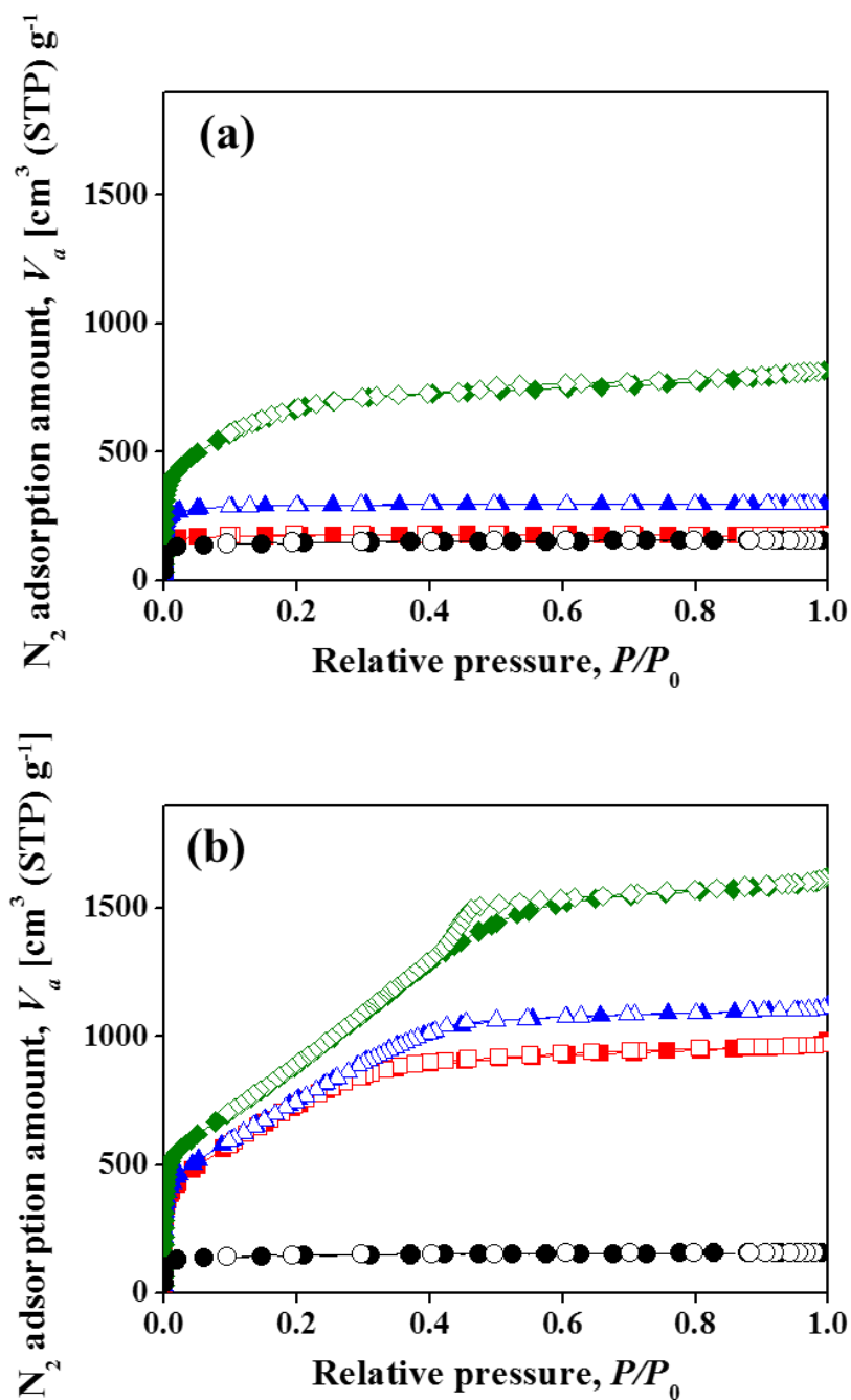
Fig. 3-1. N_2 adsorption/desorption isotherms at 77 K of C6 and (a) steam- and (b) KOH-activated carbons (ACs). The solid and open symbols denote adsorption and desorption isotherms, respectively. (Circle) C6; (square) C6S7 or C6K7; (triangle) C6S8 or C6K8; (diamond) C6S9 or C6K9. ("Reprinted from Journal of Carbon, 114 / 4015720288522, Doo-Won Kim, Hyun-Sig Kil, Koji Nakabayashi, Seong-Ho Yoon, Jin Miyawaki, Structural elucidation of physical and chemical activation mechanisms based on the microdomain structure model, 98-105, 2017, with permission from Elsevier.")
