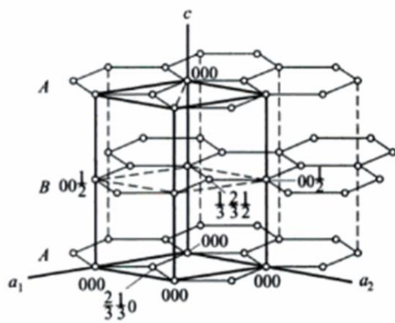
Hexagonal graphite
