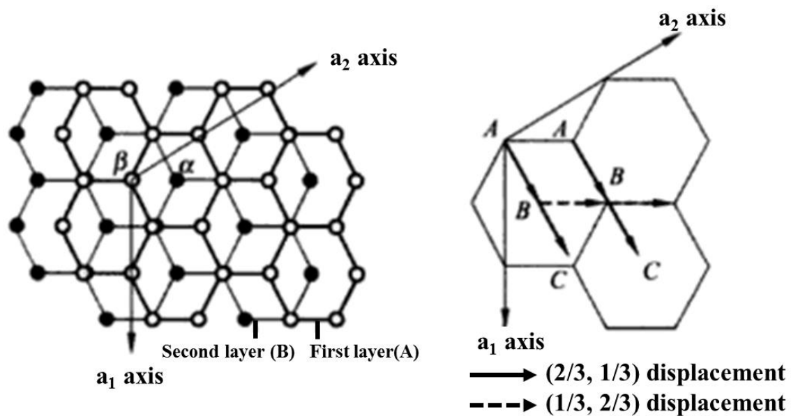
Graphite structure
