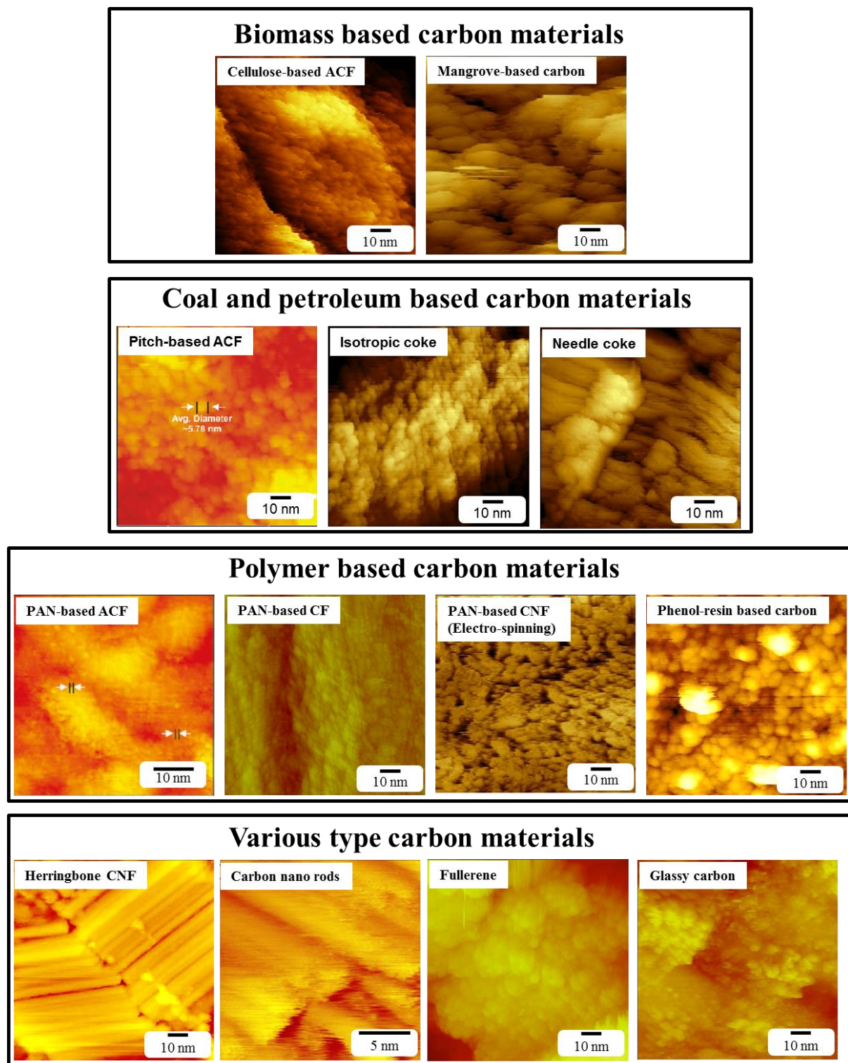
Fig. 2-1. Microdomain structures of various carbon materials. (To express of information about rights and permissions of some images in the acknowledgements)
