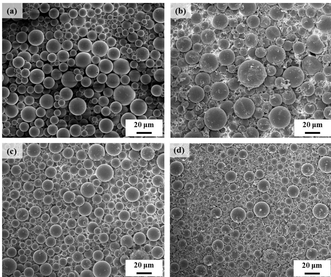
Fig. 5-1. Scanning electron microscopy (SEM) images of (a) C6, (b) C6K9, (c) C6-H2800, and (d) C6K9-H2800.
