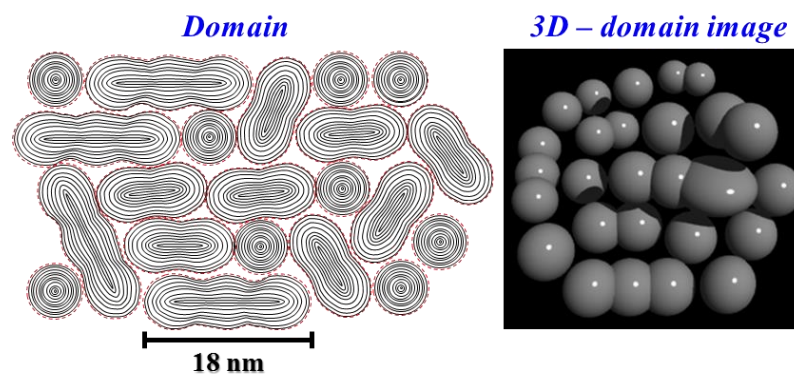
SPR-C6A9G (Graphitized graphitizable carbon)
