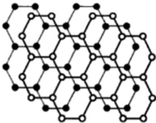
Turbostratic structure
