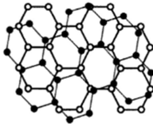
Turbostratic structure
