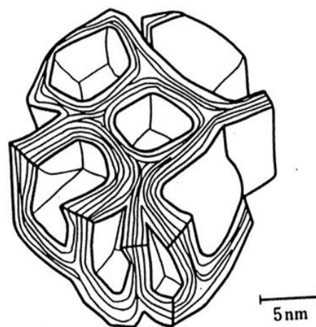
Shell model
