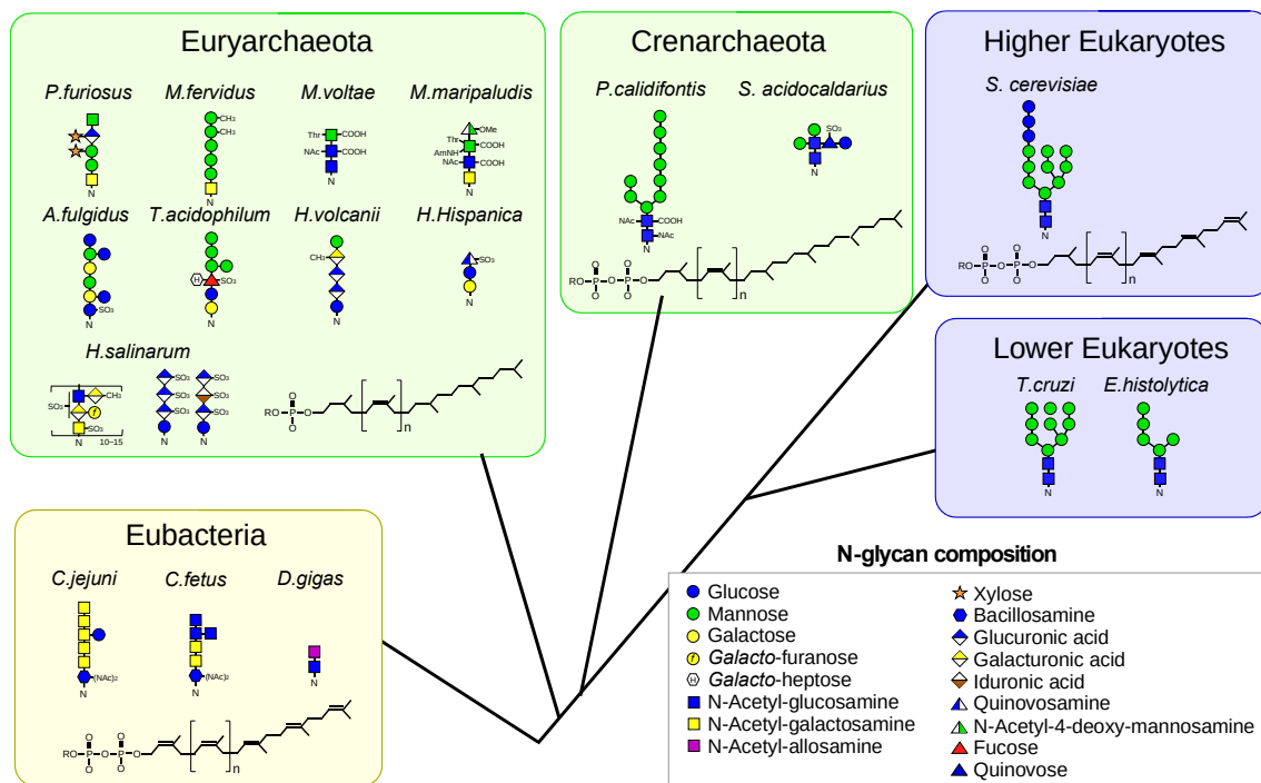
Figure 1-2. The N-linked oligosaccharide and lipid carrier structures in archaea and eubacteria species.
