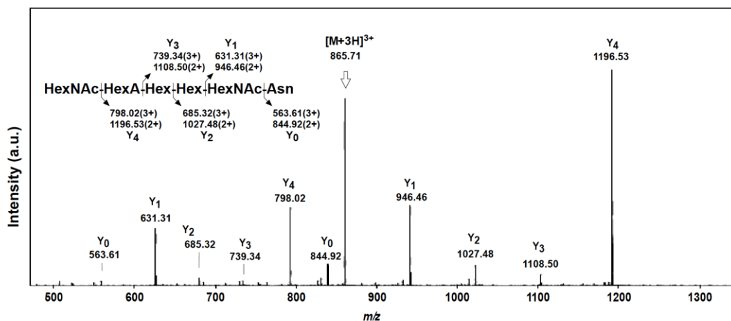
Figure 2-2. ESI-MS/MS analyses of glycopeptides P1 and P3. The precursor ions are marked by the vertical arrows. Assignments of the MS/MS fragment ions originating from single cleavages are illustrated as insets. The [M+2H]^{2+} and [M+3H]^{3+} ions are marked with 2+ and 3+, respectively. The fragment ions derived through double cleavages are shown in the spectrum, in addition to the single cleavage products. The expected m/z values were observed within 0.01.
