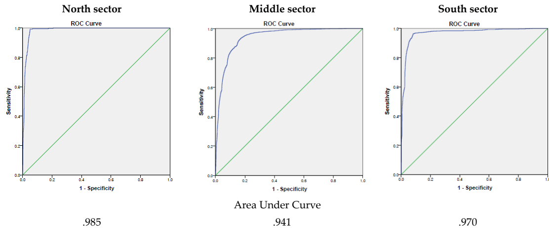
Figure 4.4 ROC curves of the logistic regression model for the three study sectors
