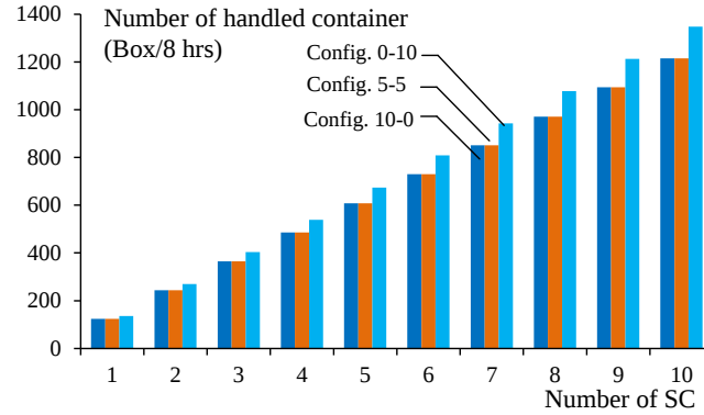
Figure 13 Transport production of SC corresponds to slot configuration
