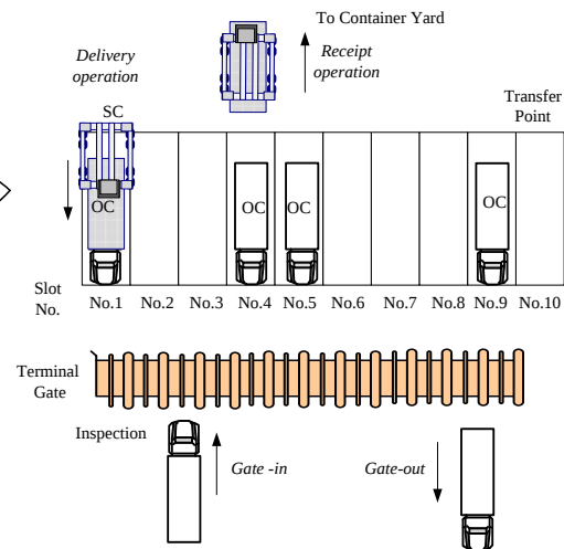
Figure 10 Flow of process for Receipt and Delivery Operation
