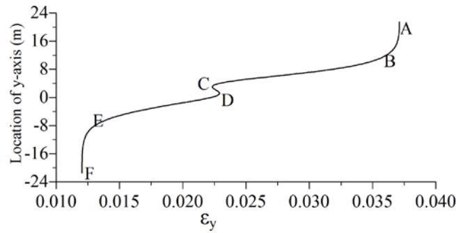
Fig.3 \varepsilon_y of soil at the center of two adjacent piles.
