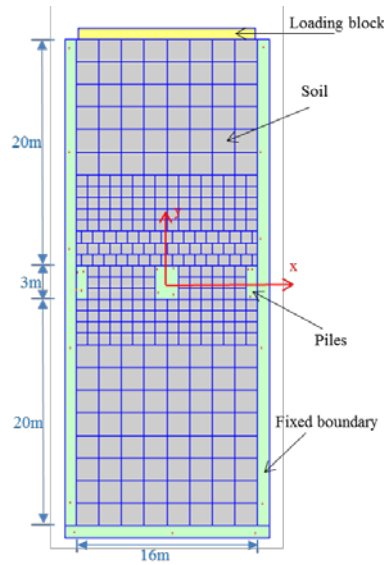
Fig.8 The numerical simulation model of DDA.
