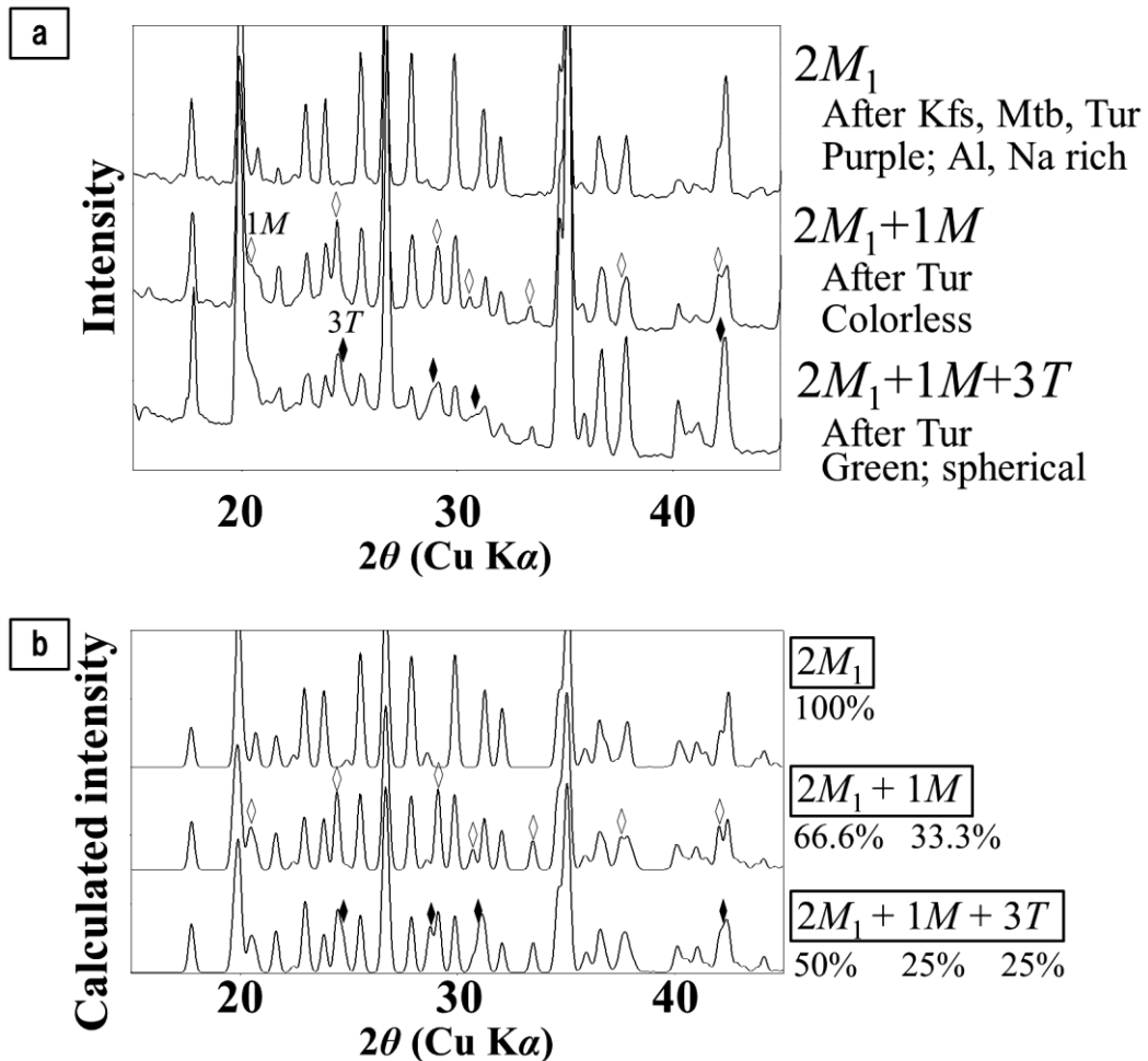
Fig. 35 X-ray diffraction patterns of muscovite composed of different polytypes. Open diamond is characteristic peak of 1M polytype, and solid diamond is that of 3T polytype. (a) Measured XRD patterns of muscovite with random orientation. Specimens are green part in Ng 114, white part in Ng10 and green part in Ng 116 in descending order. (b) Calculated XRD patterns of muscovite with mixed polytypes, referenced as follows; 2M_1 (Liang & Hawthorne 1996), 1M (Plançon et al. 1985), and 3T (Güven & Burnham 1967).
