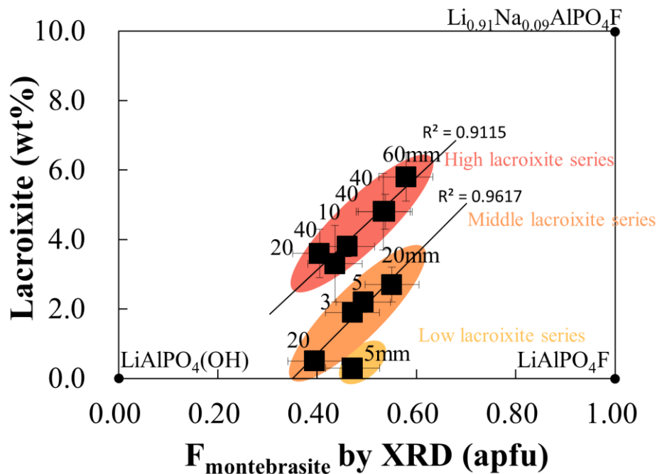
Fig. 20 Fluorine contents ( apfu ) versus lacroixite contents (wt%) of montebrasite and amblygonite from Nagatare Li pegmatite, estimated by XRD patterns (Shirose & Uehara, in press). The values on symbols indicate grain size. The bars indicate standard deviations.
