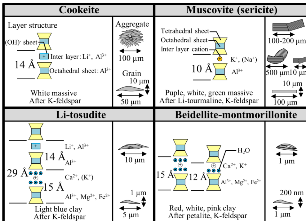
Fig. 54 Detailed mineralogical properties of clay minerals formed by alteration of primary minerals from the Nagatara pegmatite.
