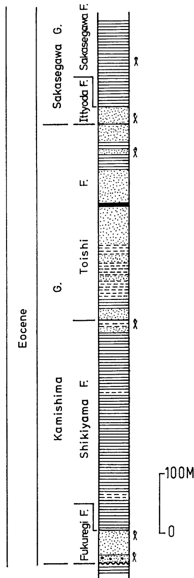
Fig. 5. Columnar section of the Paleogene in Amakusa-Shimoshima.
