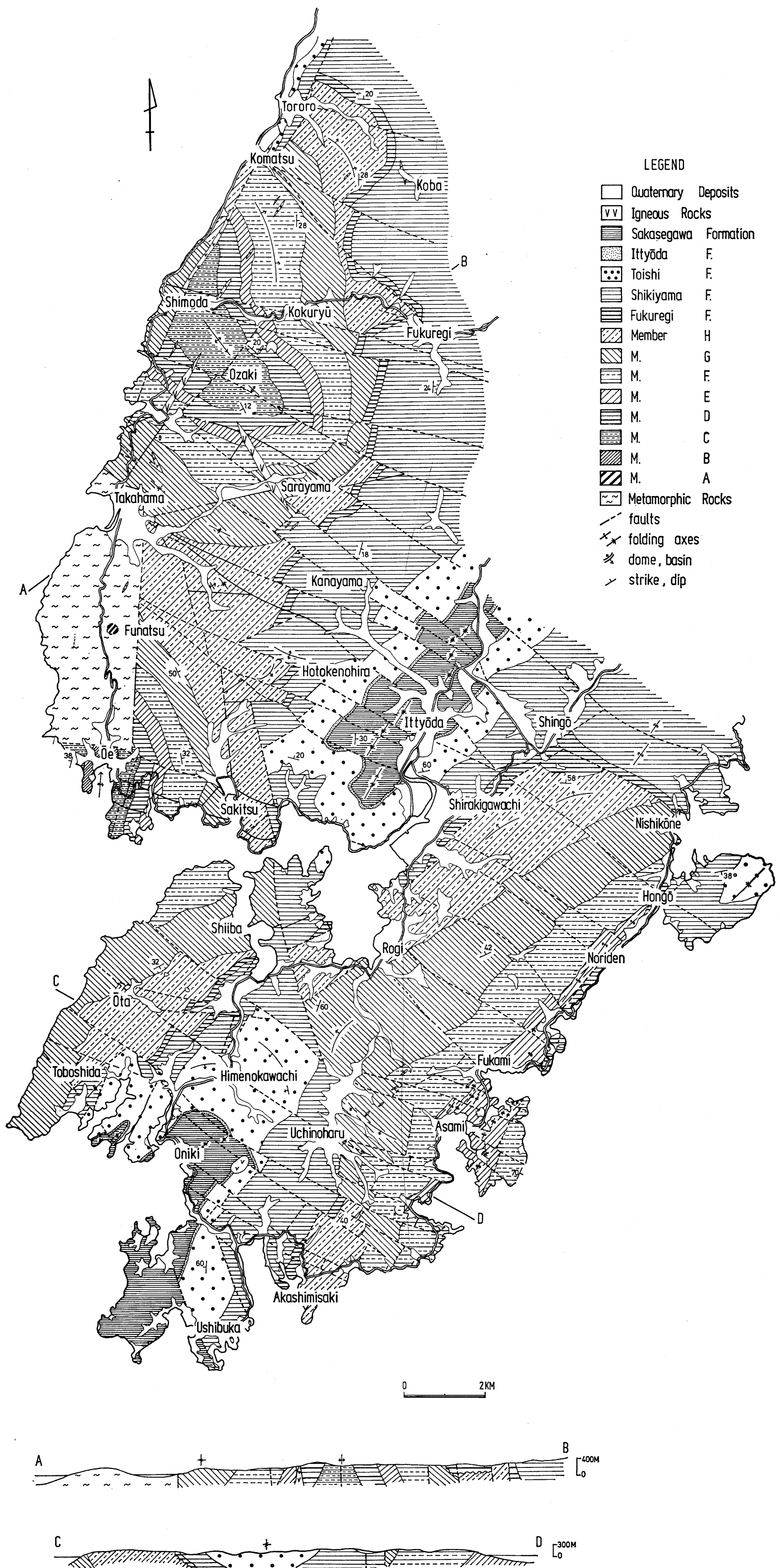
Fig. 2. Geological map of Amakusa-Shimoshima.
