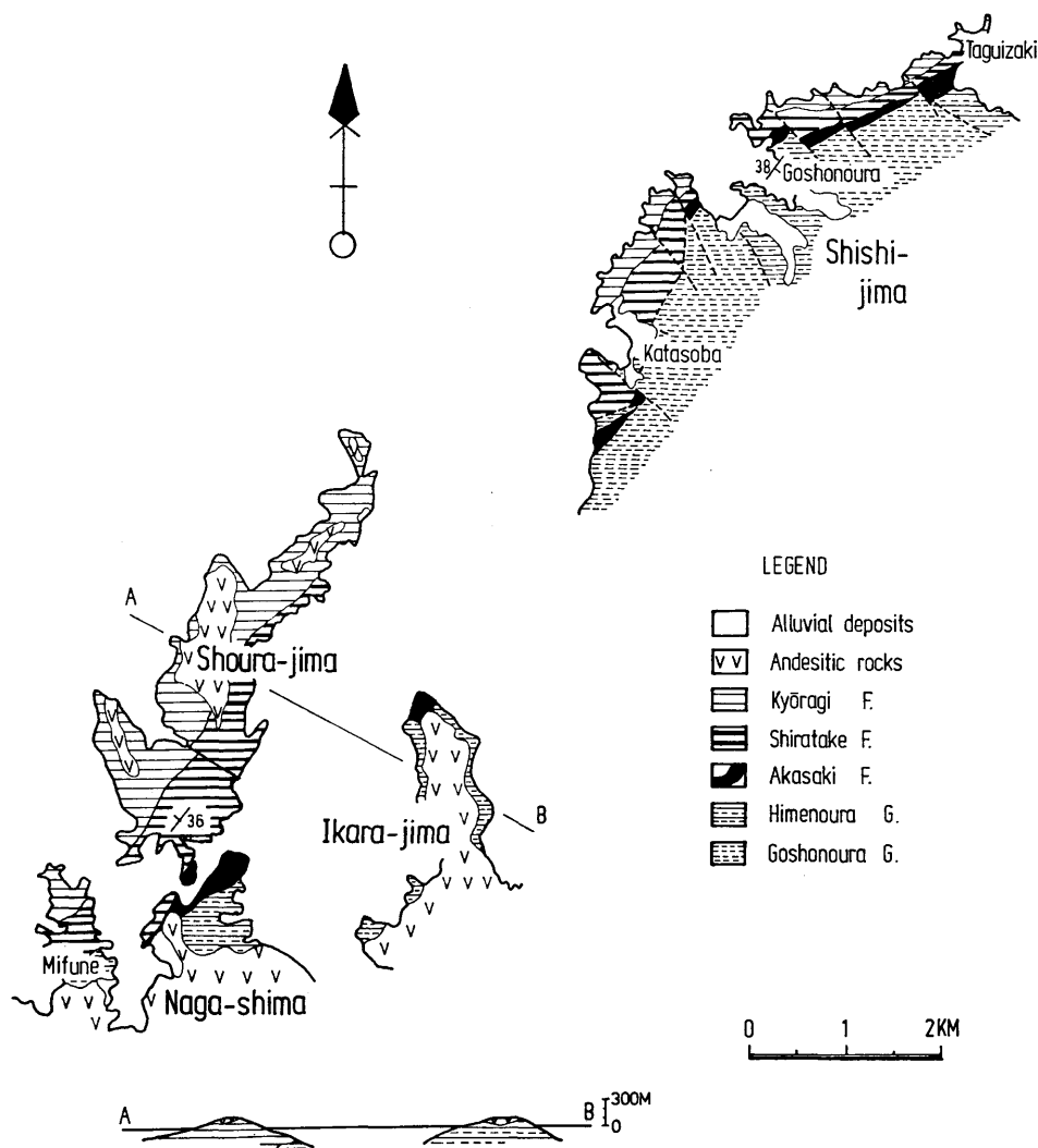
Fig. 10. Geological map of Shishi-jima and Naga-shima.
