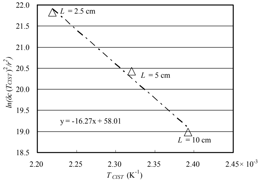
Figure 5- 3 Plotting \ln(\delta_c(T_{CSIT})^2/r^2) against (T_{CSIT})^{-1} based on critical
