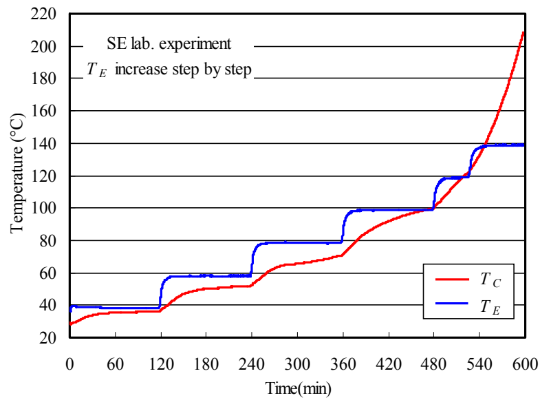
Figure 3- 5 Center temperature-time increase curve of SE (sub-bituminous)
