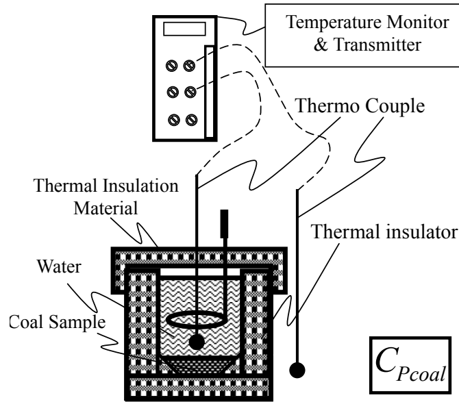
Figure 2- 6 Specific heat capacity of coal samples measurement
