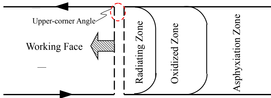
Figure 5- 4 Schematic of three zones in the goaf
