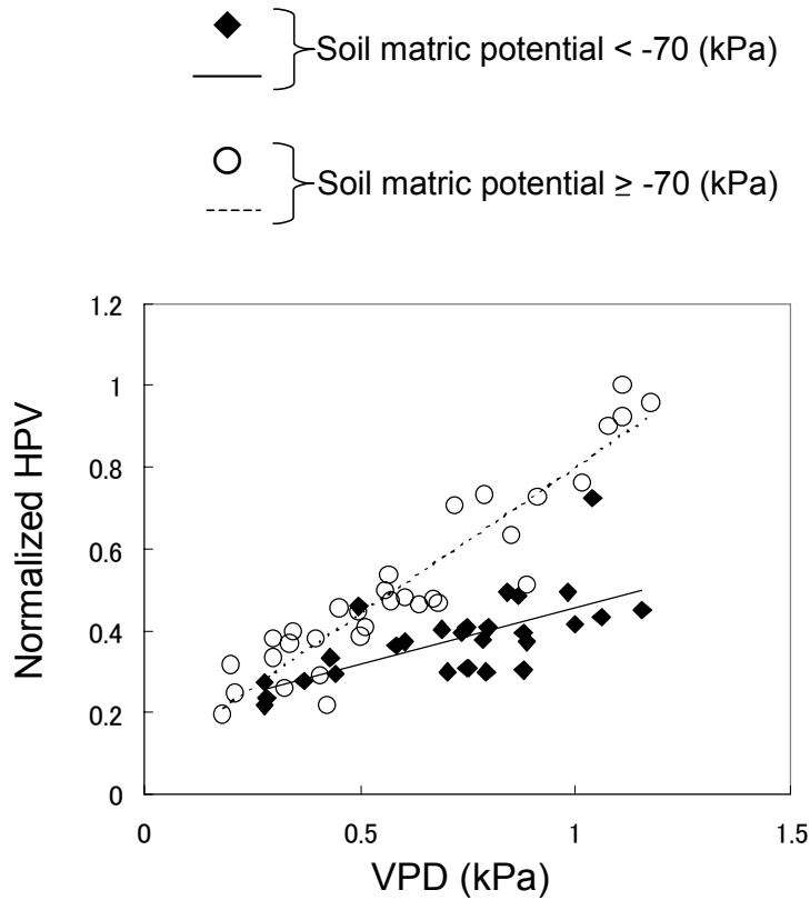
Fig. 2. Relationship between vapor pressure deficit (VPD) and normalized heat-pulse velocities (HPVs) classified according to soil matric potential (average of data from Observation Points 1 and 2).
