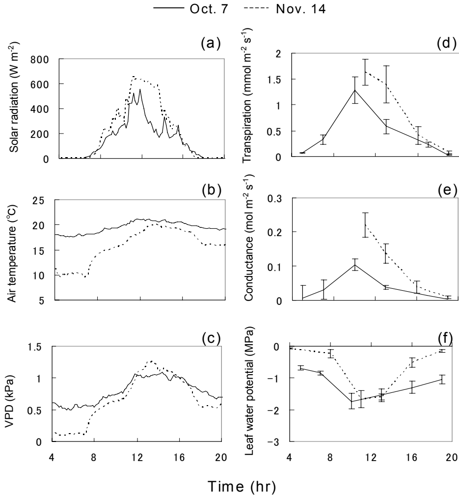
Fig. 3. Diurnal course of (a) solar radiation, (b) air temperature, (c) vapor pressure deficit (VPD), (d) leaf transpiration rates, (e) leaf stomatal conductance, and (f) leaf water potential on October 7 and November 14. Leaf transpiration rates and stomatal conductance were not measured in the early morning of November 14 due to heavy dew. October 7 was in the period with heat-pulse velocity reduction, while November 14 lies outside the period.
