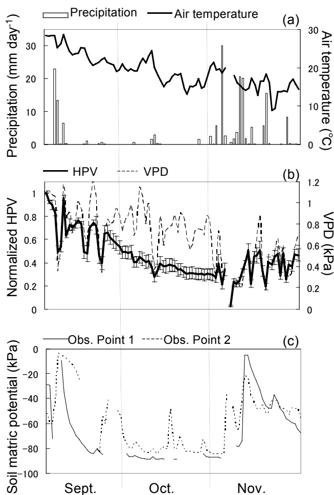
Fig. 1. Meteorological conditions, daily heat-pulse velocities (HPVs), and soil matric potential at a 10 cm depth. (a) Precipitation and air temperature; (b) HPVs and vapor pressure deficit (VPD); (c) soil matric potential at two observation points in the forest. HPV values were normalized by the value on September 6 (i.e. the first day of sap flow measurements) and averaged for the number of sample trees ( n = 6 ). Vertical bars indicate standard deviation.
