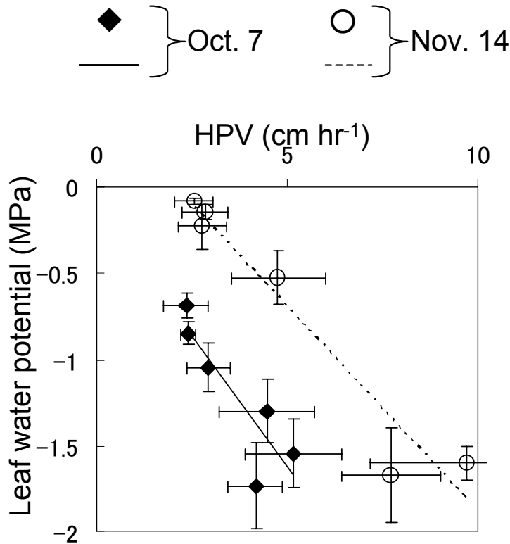
Fig. 4. Relationship between heat-pulse velocities (HPVs) and leaf water potential on October 7 and November 14. October 7 was in the period with heat-pulse velocity reduction while November 14 lies outside the period. Bars indicate standard deviation.
