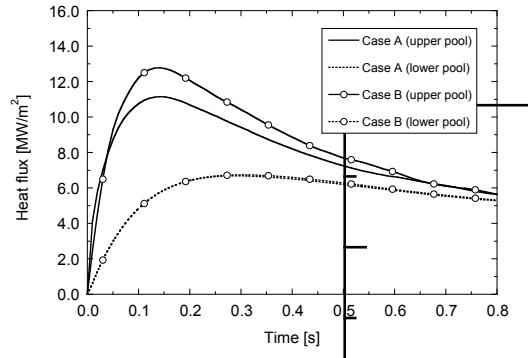
Fig. 9 Time variations of upper- and lower-pool heat fluxes in Cases A and B.
