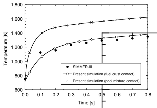
Fig. 4 Duct-wall surface temperature after the start of pool-wall heat transfer.
