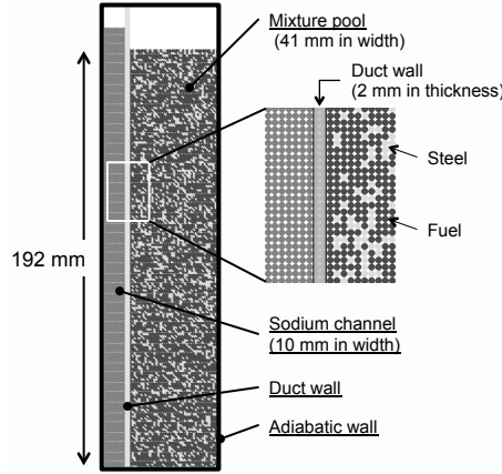
Fig. 3 Geometrical conditions for molten pool simulation.
