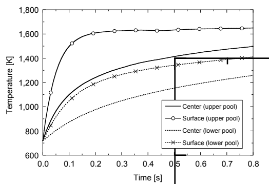
Fig. 15 Time variations of duct wall temperatures in Case C.
