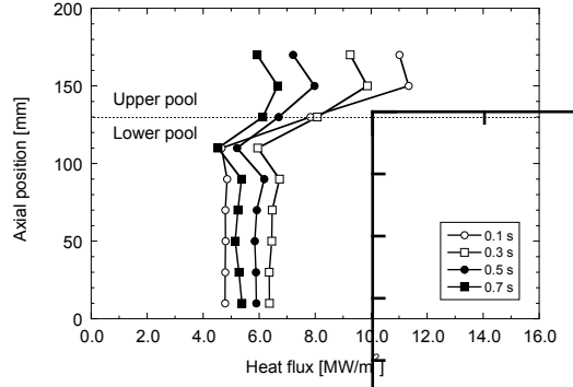
Fig. 17 Axial distributions of spatial average heat fluxes in the case of larger steel droplets.
