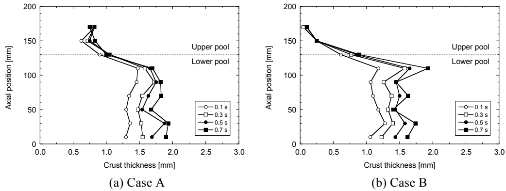
Fig. 13 Axial distributions of spatial-average crust thickness in Cases A and B.
