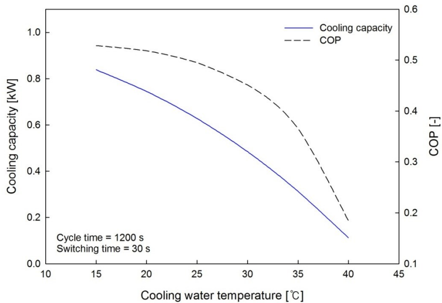
Fig. 4.9 Cooling water temperature effect on cooling capacity and COP.
