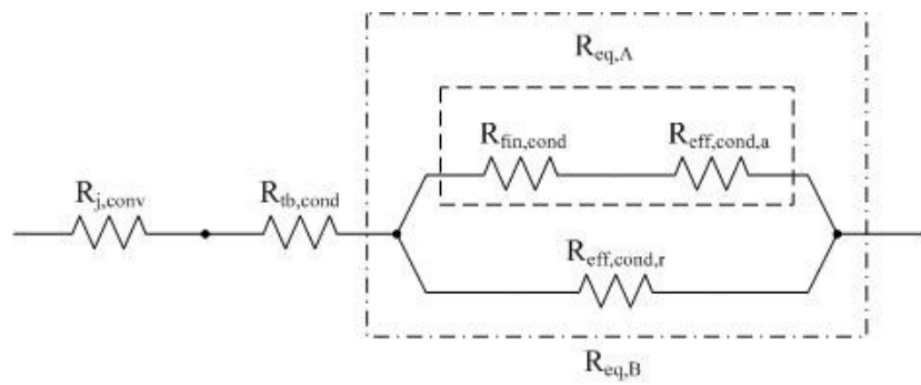
Fig. 4.2 Configuration of incremental thermal analysis.
