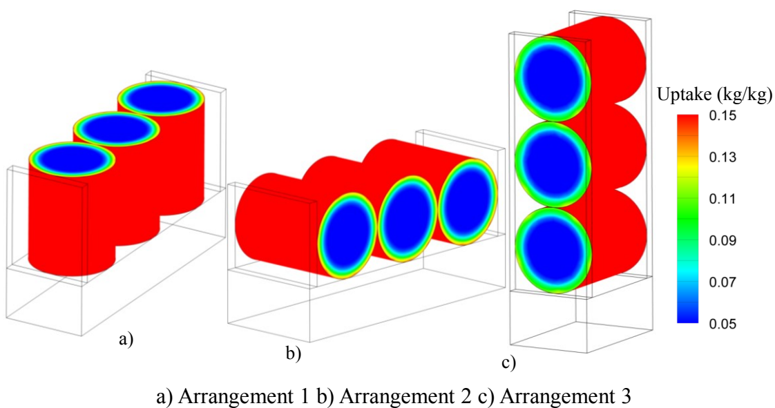
Fig. 2.11 Uptake contours on the surface and cross section.
