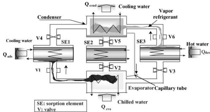
(a) Single-stage three-bed adsorption cycle in parallel heat transfer fluid flow configuration.
