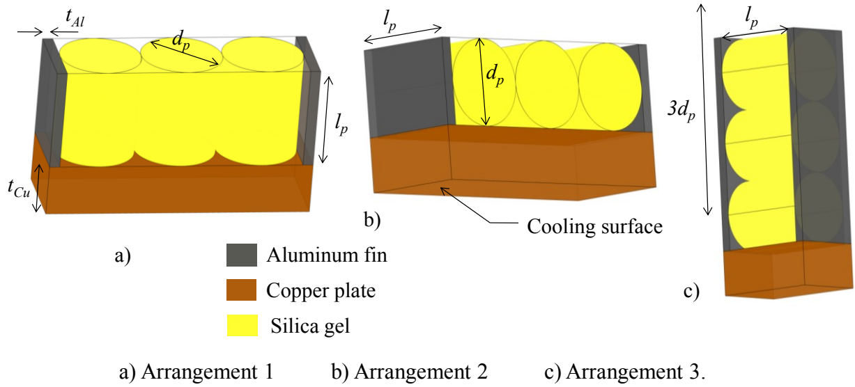
Fig. 2.9 Three different arrangements of silica gel particles.
