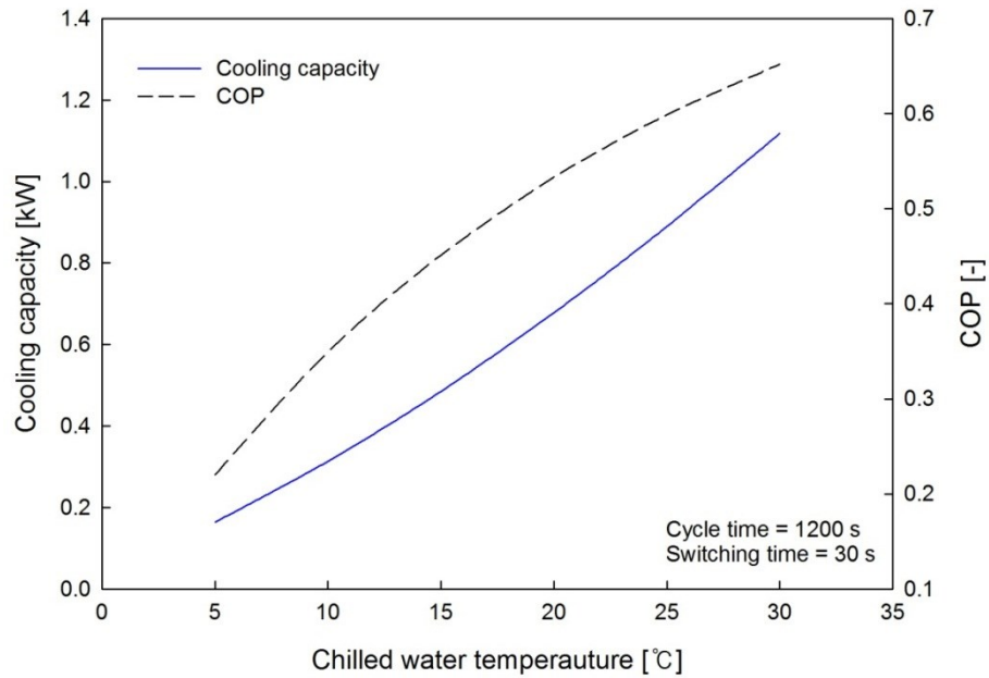
Fig. 4.10 Chilled water temperature effect on cooling capacity and COP.
