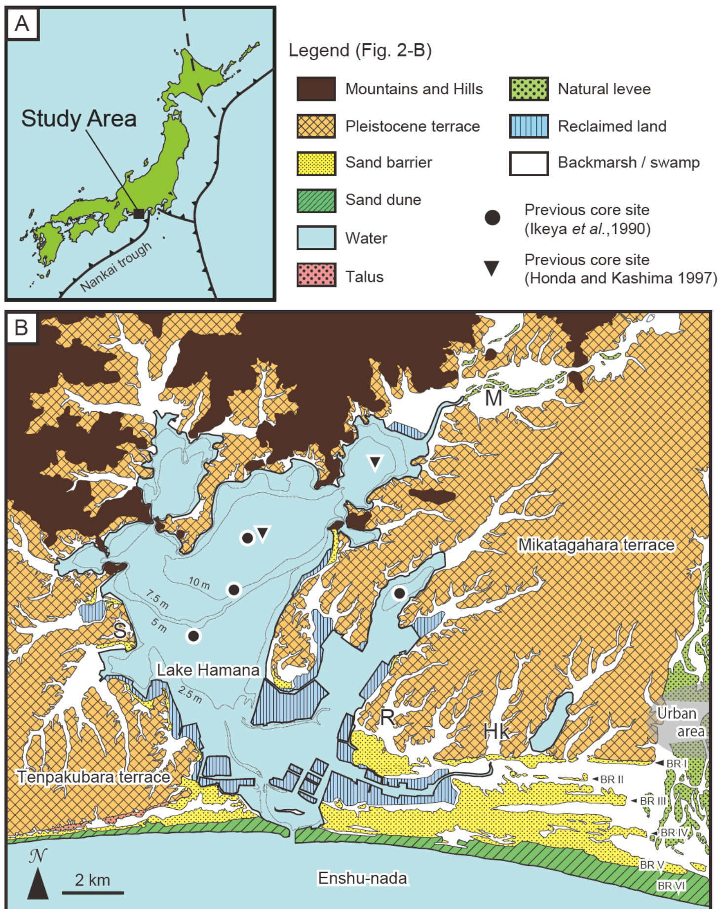
Fig. 2-1. Location and geomorphological classification map of the study area. 2-1A: Location map of the Lake Hamana. 2-1B: geomorphological classification map around the study area based on the observation of aerial photos on a scale of 1/10,000 taken by Geospatial Information Authority of Japan (GSI) in 1962. Bathymetric data is based on the topography map described in 2007 by the GSI. The urban area was changed artificially too much associated with civilization of Hamamatsu city to identify original topography. Locations of the lake bed core analyzed by previous studies (Ikeya et al. , 1990; Morita et al. , 1998) are described. R, Hk, M and S letters represent investigated alluvial lowlands in the present study, R: Rokkengawa; Hk: Higashi-Kandagawa; M: Miyakodagawa; S: Shinjo Lowlands.
