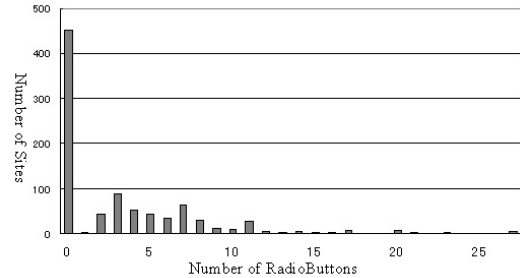
Fig. 4 The number of RadioButtons in books search sites
