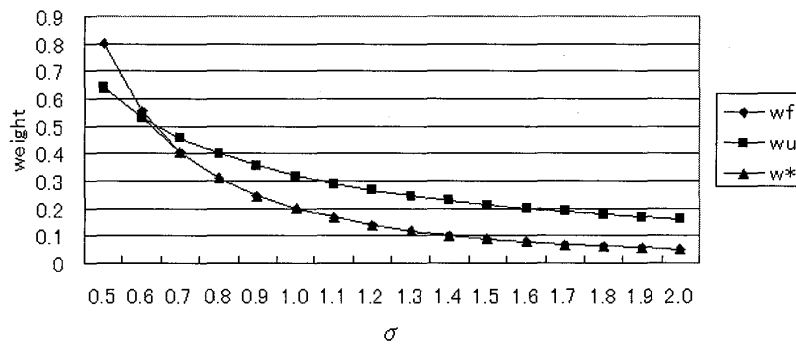
Figure 1: Change of w^* along \sigma
